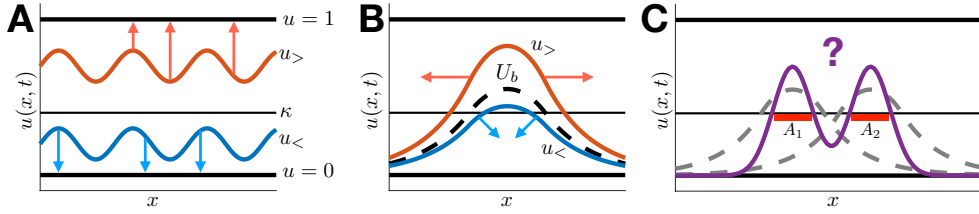
FIG. 1. Long term behavior of initial conditions u_0(x) for Eq. (1) in 1D. (A) Entirely sub-threshold (superthreshold) initial conditions decay (grow). If u_0(x) < \kappa, \forall x , then u \rightarrow 0 as t \rightarrow \infty ( u_< ), whereas if u_0(x) \geq \kappa, \forall x , then u \rightarrow 1 as t \rightarrow \infty . (B) Initial conditions below (above) the unstable bump U_b(x) decay (grow). If u_0(x) < U_b(x), \forall x , then u \rightarrow 0 as t \rightarrow \infty ( u_< ), whereas if u_0(x) > U_b(x), \forall x , then u \rightarrow 1 as t \rightarrow \infty . (C) Characterization of \lim_{t \rightarrow \infty} u(x, t) is less straightforward for multimodal initial conditions. Even though each active region ( A_1 and A_2 , where u_0(x) \geq \kappa ) is narrower than the unstable bump U_b(x) , this initial condition could lead to propagation due to nonlocal interactions.
