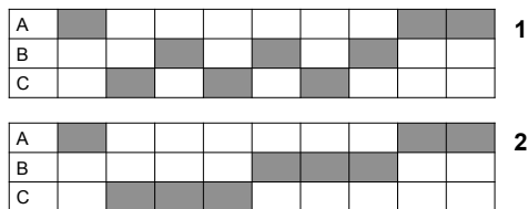
Figure 1: Two solutions of an assignment problem, A, B and C are machines and gray cells are tasks.
