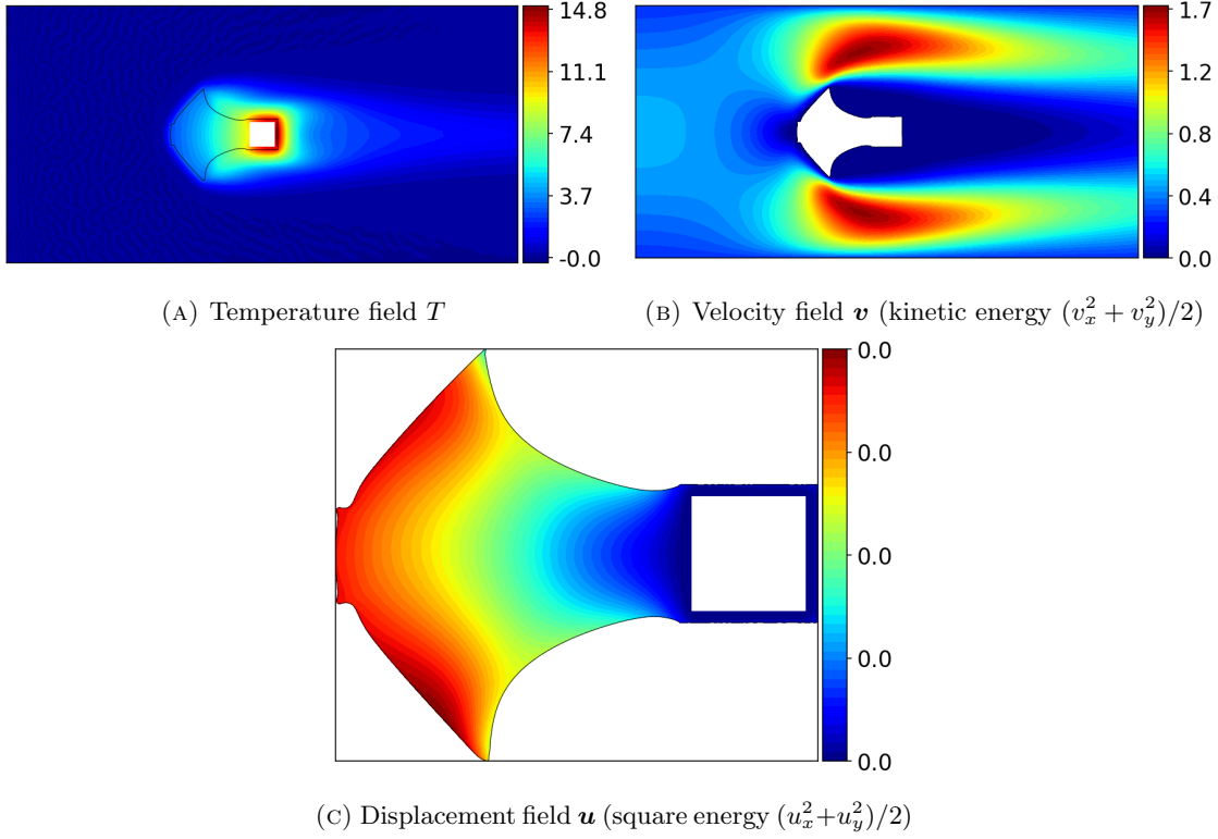
FIGURE 19. State variables \mathbf{v} , T and \mathbf{u} for the optimized configuration of the three-physic shape optimization problem of Section 6.4, in the situation h > 0 and solved with the Navier-Stokes equations.
