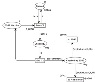
Figure 5: Explosive detection system
