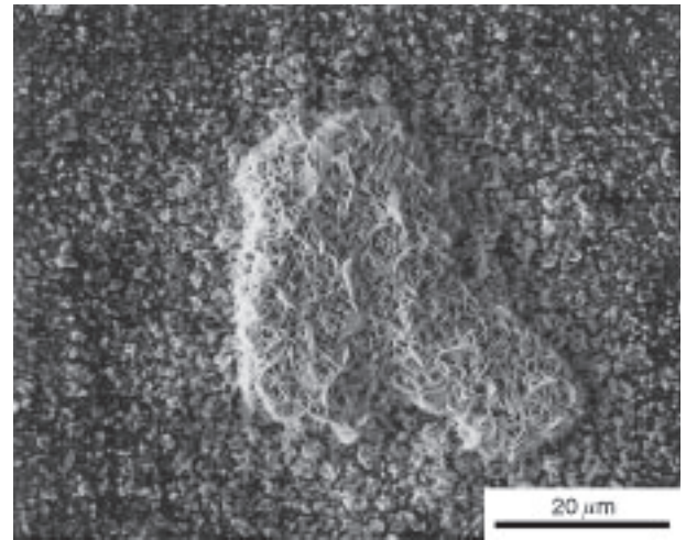
Figure 5 Scale morphology of specimen after 200 h isothermal oxidation at 880 °C.
