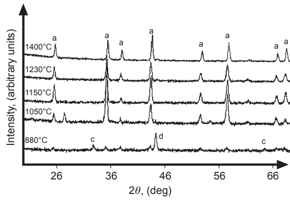
Figure 2 X-ray diffraction results (a = \alpha -Al 2 O 3 , c = \theta -Al 2 O 3 , d = Fe).
