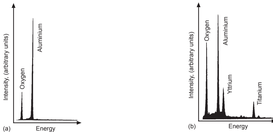
Figure 4 EDX analysis of specimen after 70 h isothermal oxidation at 1150 °C, (a) flat base scale, (b) overlying nodule.
