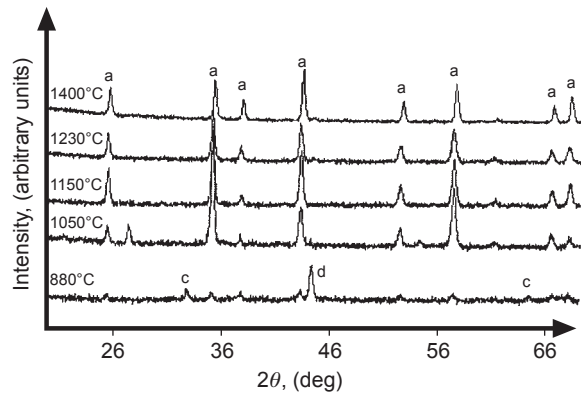
Figure 2 X-ray diffraction results (a = \alpha -Al 2 O 3 , c = \theta -Al 2 O 3 , d = Fe).
