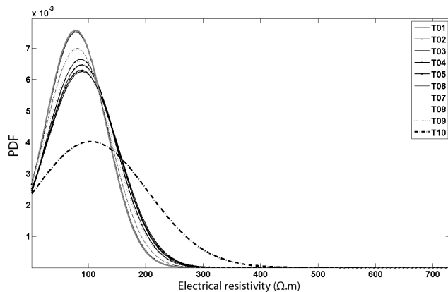
Figure 3. Probability density functions (PDF) estimated from electrical resistivity measurements of the entire 2-D section at each date of electrical resistivity tomography. Curves were fitted with a Gaussian model.
