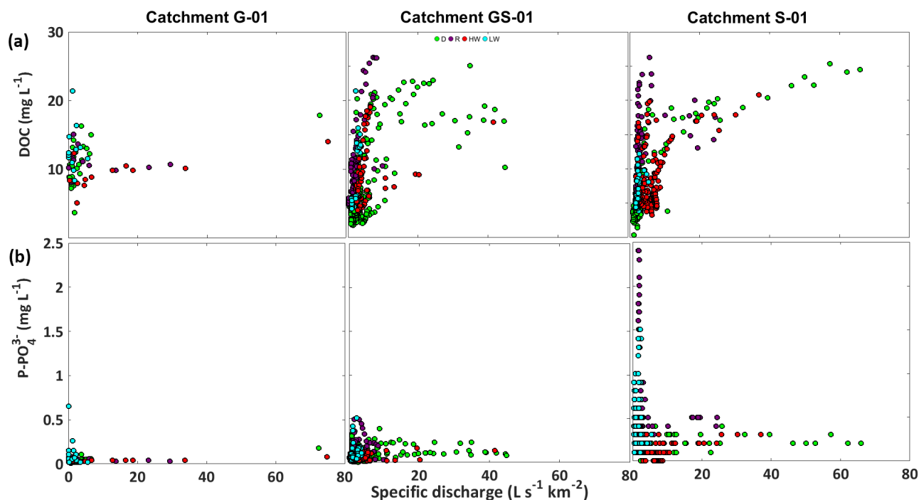
Figure 2. Relationship between specific discharge and (a) dissolved organic carbon, on the one hand, and (b) phosphate, on the other hand, for three headwater catchments (G-01, GS-01, and S-01) in Brittany, France. Chemistry data from daily automatic sampling supplemented by sub-daily sampling for catchments GS-01 and S-01 during discharge events (see methods for detailed sampling description). Data are colored by hydrologic period: D – discharge (April–June); LW – low water (July–September); R – recharge (October–December); HW – high water (January–March).
