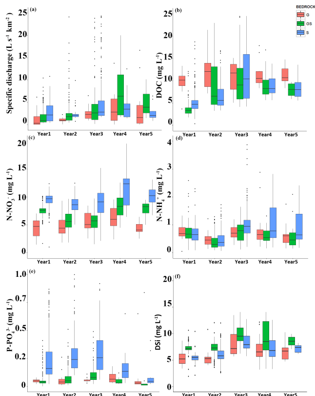
Figure 5. Discharge and carbon and nutrient concentrations during 5 contrasting hydrological years. Boxplots of (a) specific discharge, (b) dissolved organic carbon, (c) nitrate, (d) ammonium, (e) phosphate, and (f) dissolved silica for the catchments G-01 (red box), GS-01 (green box), and S-01 (blue box). Boxplots represent median, quartiles, minimum, and maximum within 1.5 times the interquartile range and outliers beyond 1.5 interquartile range.
