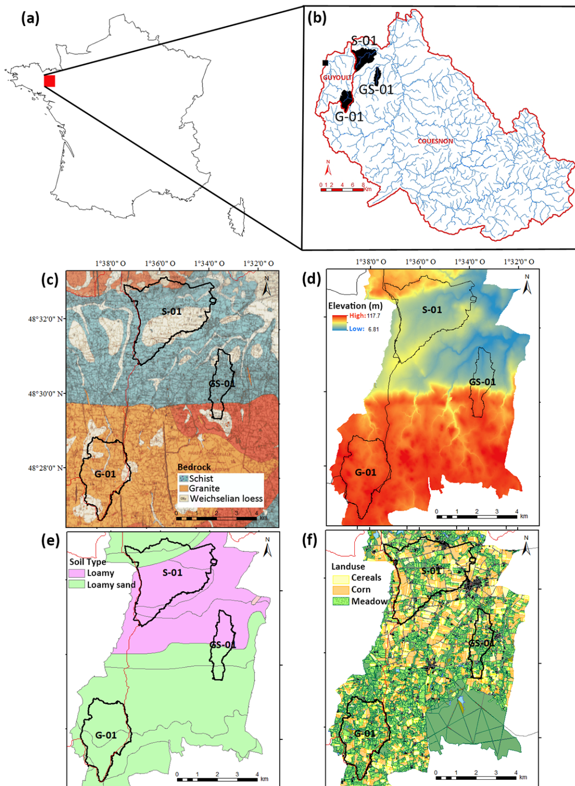
Figure 1. Location and physical characteristics of the three study catchments. Panel (a): the red square delineates the Zone Atelier Armorique LTER on the map of France. Panel (b): the catchment G-01 is a subcatchment of the Le Guyoult basin (gauged outlet indicated by black square). The two catchments GS-01 and S-01 are subcatchments of the Couesnon basin. Panel (c): geological overview showing granite in the south and schist in the north. Panel (d): digital elevation model from lidar with a 2 m resolution; elevation given in m.a.s.l. Panel (e): land use from the last year of study period (i.e., 2000). Panel (f): map of soil type.
