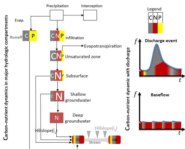
Figure 6. Conceptual model of carbon and nutrient dynamics in major hydrologic compartments during transient (discharge events) and steady-state (baseflow) discharge regimes. On the left side, we represent the relative abundance of carbon, nitrogen, and phosphate during vertical transport through soil, unsaturated zone, and groundwater. Arrows represent flow paths, which can either descend through the soil column or lead directly to the stream (represented at the bottom of the figure), which experiences fluctuations in water chemistry based on the relative contribution of these flow paths from multiple hillslopes. On the right side of the figure, schematic representations of stream chemistry during stormflow and baseflow are shown. The colors represent carbon, nitrogen, and phosphorus concentrations, which vary depending on hydrologic conditions. See Sect. 4.2 in the “Discussion” section for more detailed interpretation.
