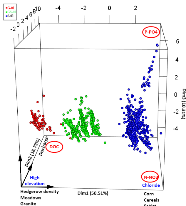
Figure 4. Principle components analysis of the major sources of variability in water chemistry. Together, the first three axes explain 80 % of the total variability of the data. Principal and supplementary variables are indicated respectively in black and blue. Red circles indicate the poles of carbon, nitrogen, and phosphorus associated with cereals and corn for \text{N-NO}_3^- , high discharge on granite bedrock for DOC, and both discharge and agricultural land use for \text{P-PO}_4^{3-} . PCA scores are indicated in Table S3.
