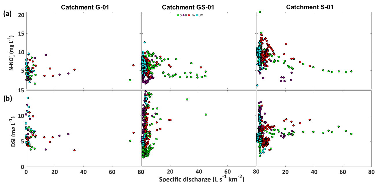
Figure 3. Relationship between specific discharge and (a) nitrate, on the other hand, and (b) dissolved silica, on the other hand, for three headwater catchments (G-01, GS-01, and S-01) in Brittany France. Chemistry data from daily automatic sampling supplemented by sub-daily sampling for catchments GS-01 and S-01 during discharge events (see “Methods” section for detailed sampling description). Data points are colored by hydrologic period (see Fig. 2 for definitions).
