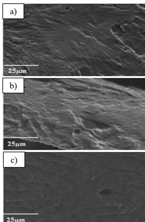
Figure 18. Cryofractured SEM micrographs of (a) pure PU, (b) PU with 3 wt% natural talc and (c) PU with 3 wt% Ni-Talc. Reprinted with permission from ref [112] .
