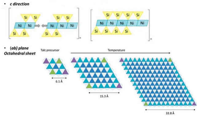
Figure 22. Scheme of the structural evolution of the talc precursor with the temperature in both the c^* direction and in the (ab) plane. Reprinted with permission from ref [128].
