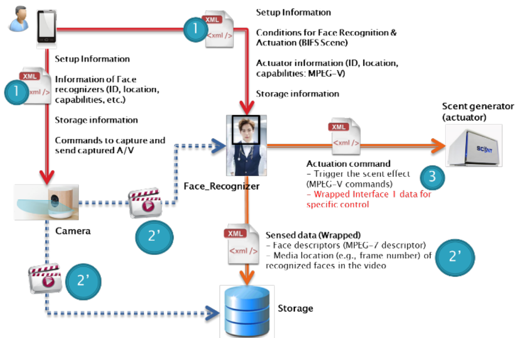
Fig. 2. Data flow schematics evoking sensorial actuations using the face detection
