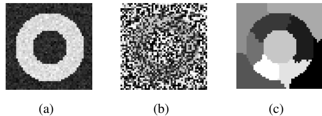
Fig. 1. An example showing that K-means does not ensure the connectivity of the clusters. (a) Original Image - Simple image with gaussian noise. (b) Clustering result obtained by using simple K- Means without any constraint on connectivity. Number of clusters is taken to be 10. (c) Clustering result obtained using the proposed algorithm 1, which performs K-Means with constraint on connectivity. Number of clusters is taken to be 10
