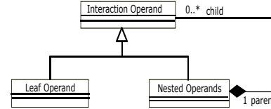
Figure 3: Interaction Operand Metamodel
