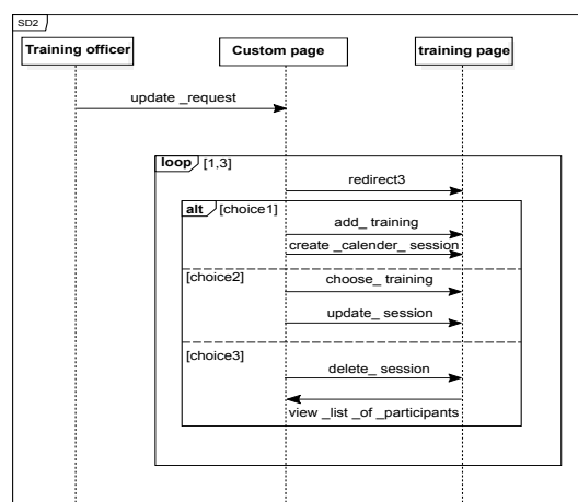
Figure 2: Update training catalog
