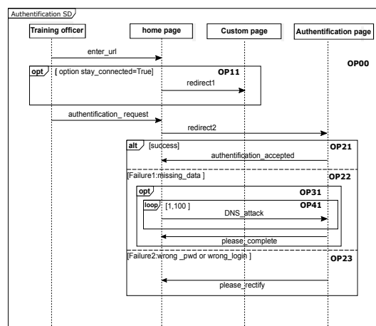
Figure 1: Authentication
