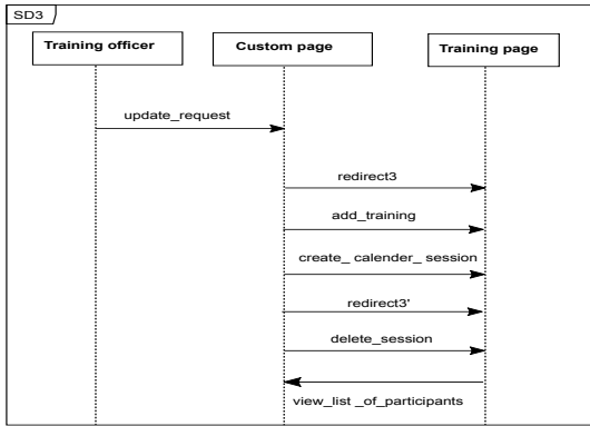
Figure 7: Possible execution of The SD of the Fig. 6
