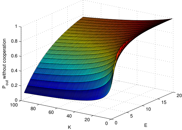
Fig. 1. PSO for the blind policy in the non-cooperative case for \tau = 1 bit/sec/Hz and diversity orders K and E .
