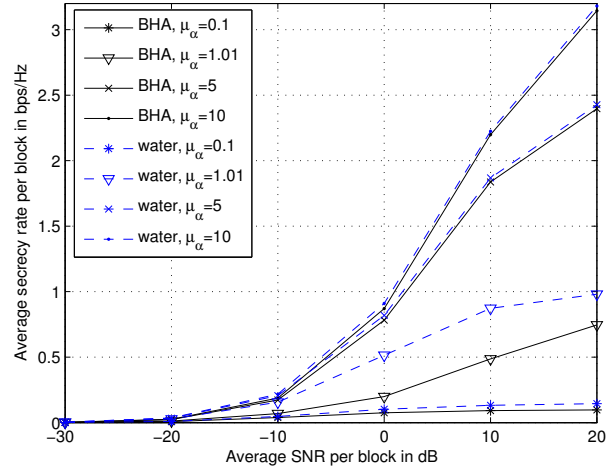
Fig. 4. Average secrecy rates achieved with causal BHA policy and acausal waterfilling policy for various policies for \mu_\beta = 1 and M = 10 .
