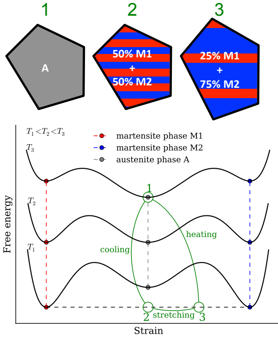
Fig. 9 Schematic representation of the physical mechanism behind the shape memory effect. Different phases of the crystalline structure exist and some can coexist because of peculiar crystallography. The phase composition is dictated by free energy minimization.
