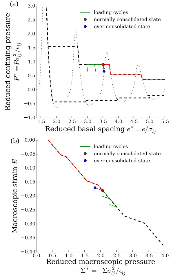
Fig. 13 Consolidation of the material by applying volumetric compression to an initial configuration at large basal spacing and moderate confining pressure. (a) Mechanical response at the scale of a stack. (b) Mechanical response at the macroscopic scale.
