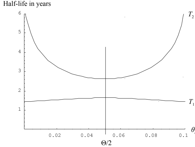
Figure 3: Half-lives.
