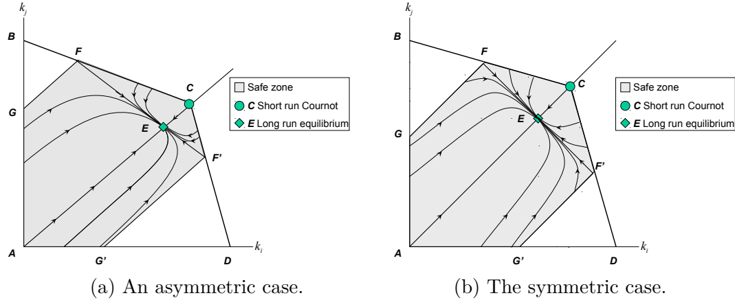
Figure 2: Trajectories.
