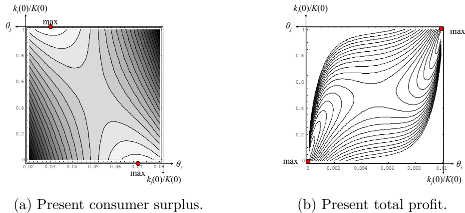
Figure 4: Synthesis.
