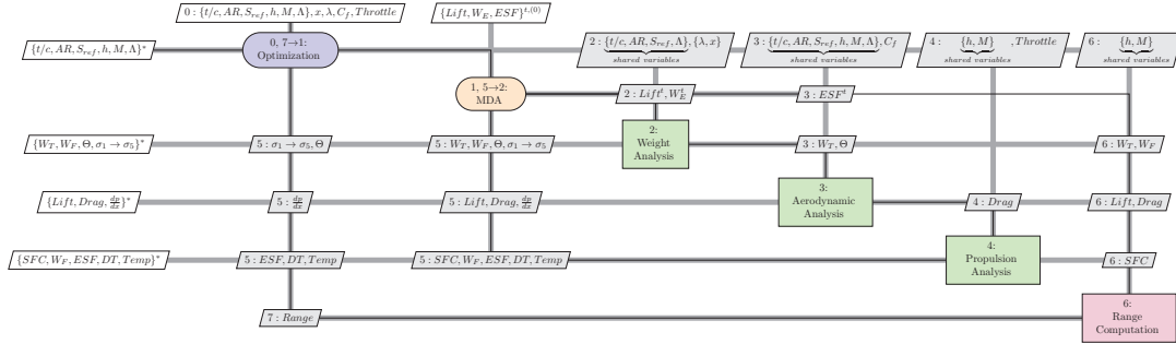
Figure 3: MDF formulation applied to the SSBJ test case
