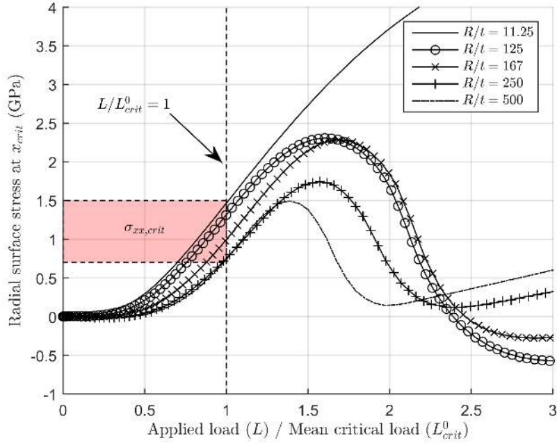
Figure 17: Evolution of the radial stress ( \sigma_{xx} ) at the surface of ALD alumina thin film as a function of the applied load, with varying ratio R/t .
