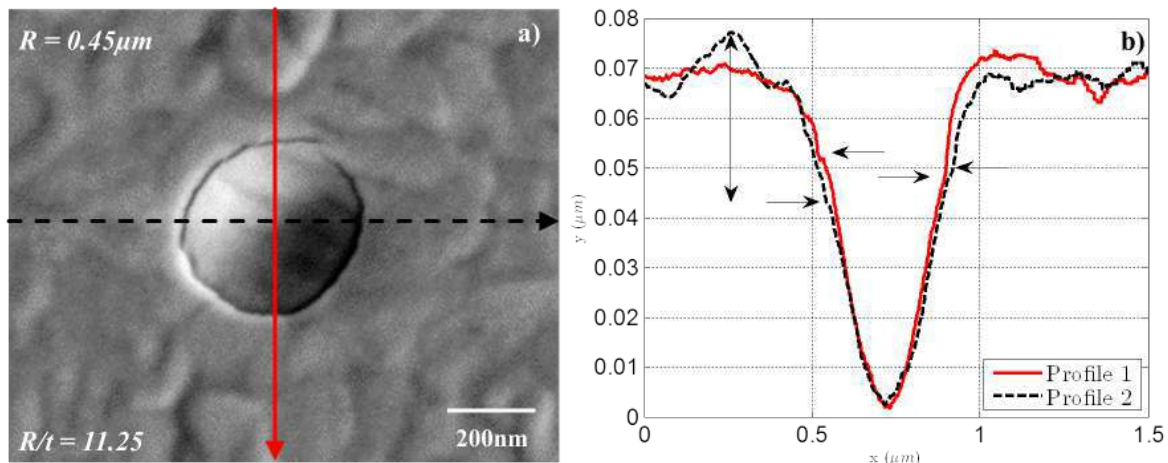
Figure 11: a) SEM observation (top view) of a residual indent in the 40nm thick ALD alumina coating with b) two height profiles obtained along the imprint topography measured by AFM.
