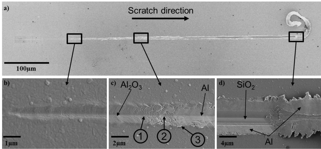
Figure 3: a) SEM observation (top view with secondary electrons) of the scratch test performed on the multilayer specimen with a 40nm thick ALD alumina coating. The different parts of the scratch experiment were magnified on the bottom part of the figure: b) start of the scratch, c) ALD alumina breakthrough and d) end of the scratch with formation of a material pile-up in front of the scratch tip.
