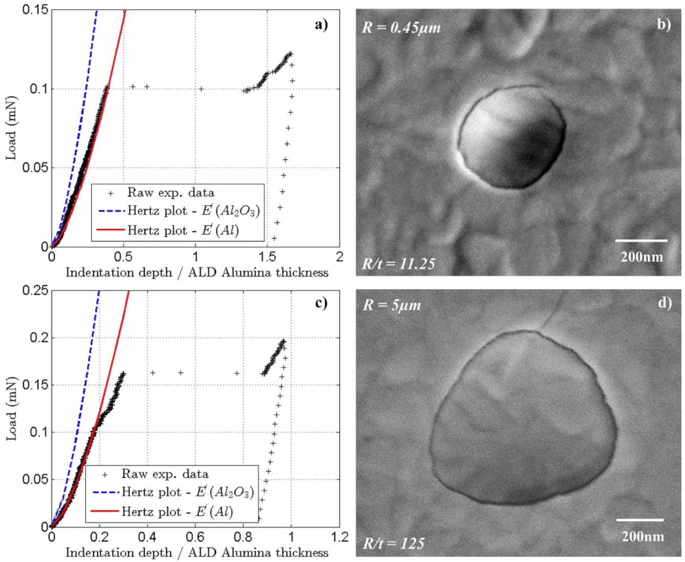
Figure 7: a) and c) are the load-displacement curves with a pop-in event and b) and d) are corresponding SEM observations (top view with secondary electrons), obtained respectively for the 0.45 \mu\text{m} and for the 5 \mu\text{m} tip radius, after spherical indentation on the 40 \text{nm} thick alumina specimen.
