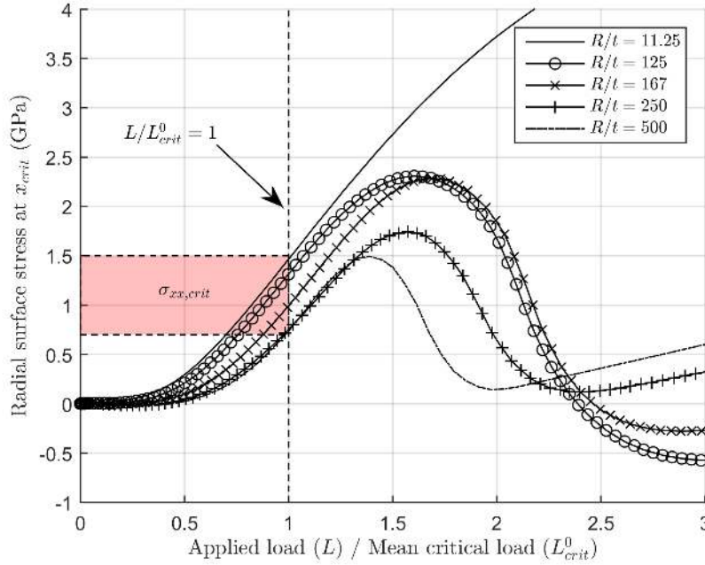
Figure 17: Evolution of the radial stress ( \sigma_{xx} ) at the surface of ALD alumina thin film as a function of the applied load, with varying ratio R/t .
