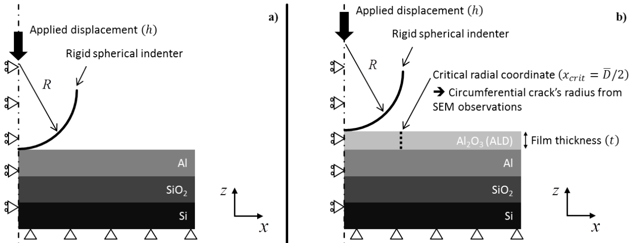
Figure 15: Schematic of the finite element modeling of spherical indentation in a multilayer sample: a) without and b) with ALD alumina coating.
