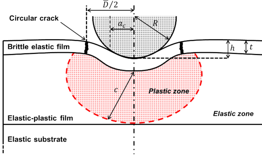
Figure 14: Schematic of spherical indentation into a brittle elastic coating on a soft elastic-plastic thin film. Here, a_c is the contact radius, R is the tip radius, c is the radius of plastic zone, \bar{D}/2 is the radius of the orthoradial crack, h is the indentation depth and t the ALD film thickness.
