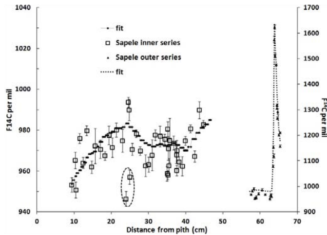
Figure 4 F^{14}\text{C} pre- and post-bomb experimental data for the sapele cross-section compared with those expected using the best-fit model.
