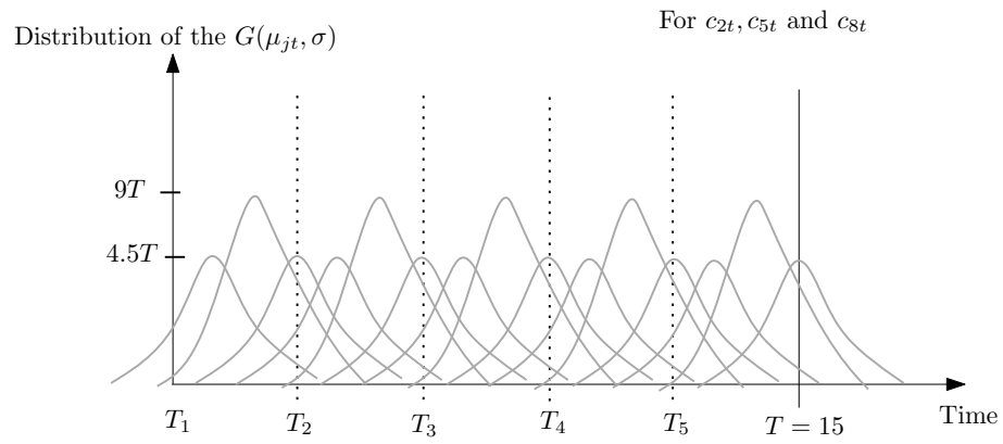
Figure 2: Example of the distribution of the processing costs with n = 9 and T = 15
