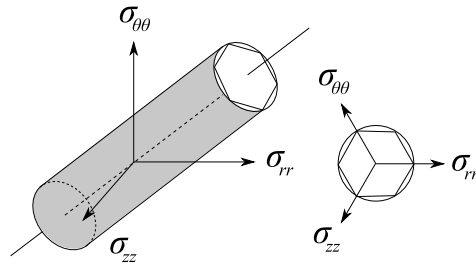
FIGURE 6 – von Mises and Tresca yield surfaces
