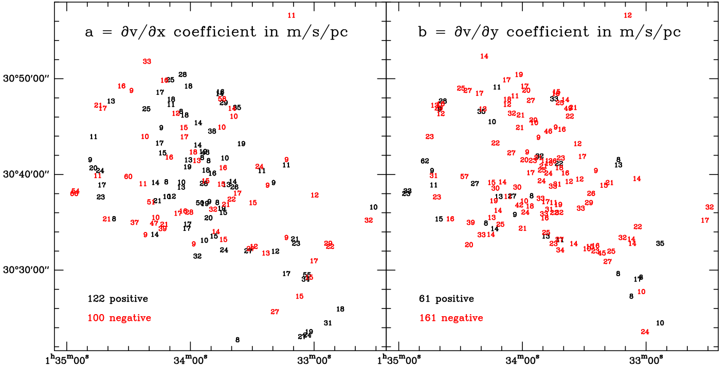
Fig. 16. Coefficients a = \frac{\partial v}{\partial RA} and b = \frac{\partial v}{\partial Dec} for the 222 stronger clouds ( T_{CO} > 0.11K ), shown only when above 8 \text{ m s}^{-1} \text{ pc}^{-1} in absolute value in order to reduce the influence of noise and make the numbers legible. Negative values are shown in red and positive in black. The numbers of negative and positive values are given in the panels. Because the panels only show the higher (absolute) values, the disproportion in the right panel is actually greater: 31 values > 8 and 116 values < -8 .
