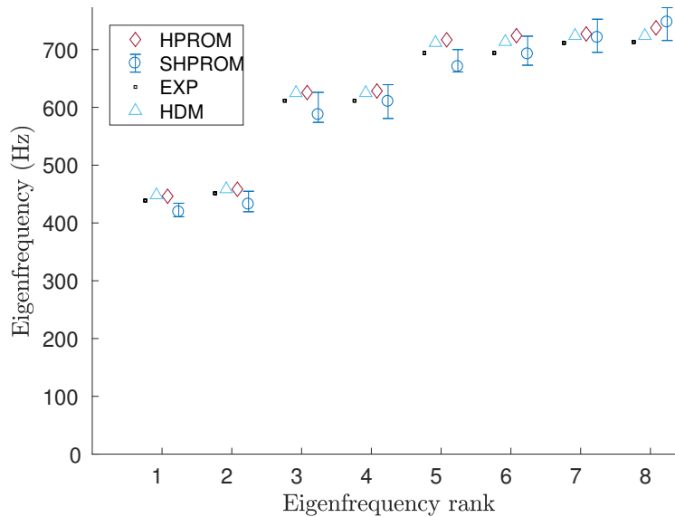
Fig. 7 Vibration analysis at (l, r) = (1.1, 1.1) : QoIs (natural frequencies) predicted using the deterministic HPRM; mean values and confidence intervals corresponding to the quantiles 98% and 2% constructed using the SHPRM; surrogate experimental values (EXP) of the QoIs; and QoIs predicted using the HDM.
