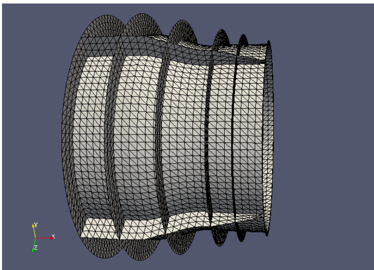
Fig. 2 Shape-parametric jet engine nozzle.
