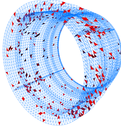
Fig. 3 Reduced mesh constructed by the ECSW hyperreduction method (sampled elements are highlighted in red color).
