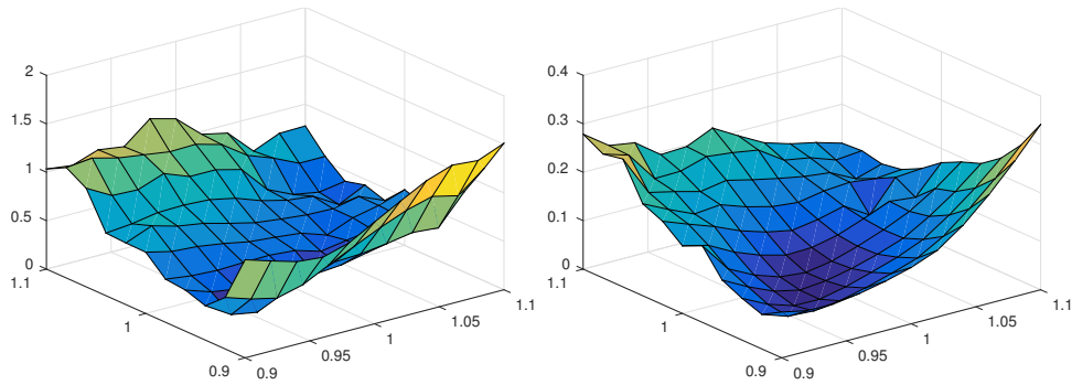
Fig. 5 Variations on an 11 \times 11(l, r) grid of the indicated (left) and true (right) HPRM errors upon declared convergence of the greedy sampling algorithm.
