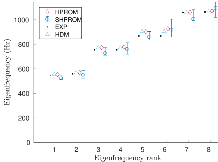
Fig. 6 Vibration analysis at (l, r) = (0.9, 0.9) : QoIs (natural frequencies) predicted using the deterministic HPROM; mean values and confidence intervals corresponding to the quantiles 98% and 2% constructed using the SHPRM; surrogate experimental values (EXP) of the QoIs; and QoIs predicted using the HDM.
