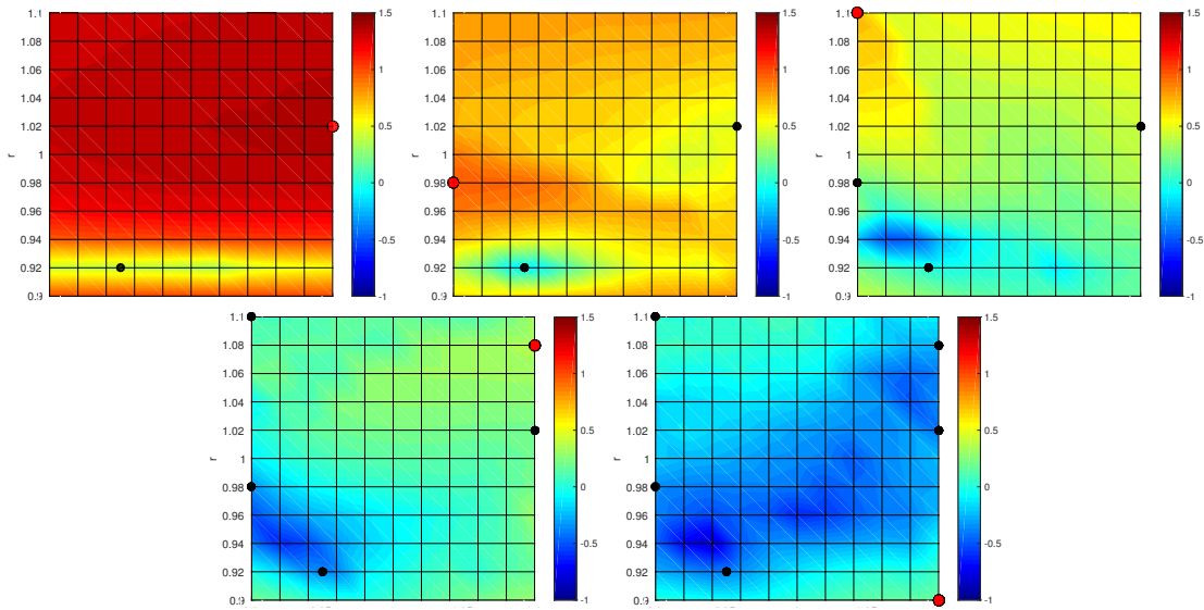
Fig. 4 Progression of the indicated error ( \log_{10} ) on an 11 \times 11(l, r) grid during the iterations performed by the greedy sampling algorithm.
