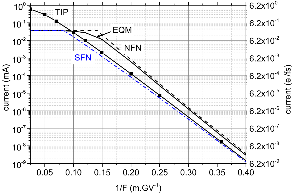
FIG. 3: State currents from state # 15 at the Fermi energy : comparison between TIP (full line+squares), EQM (full line), NFN (dashed line) and SFN (dashed-dotted line) results. Currents are given in mA (left scale) and in number of electrons per femtosecond ( e^-/\text{fs} , right scale). The SFN result is obtained from eq. 6 and eq. 11, it corresponds to the potential energy given by eq. 10. The EQM and NFN results are obtained from eq. 6 and corresponding tunneling probabilities (see subsection IIC) for the one-dimensional numerical potential energy obtained from VASP calculations (see subsection IIIB). The TIP result is obtained from eq. 14, also for the 1D potential energy extracted from VASP results.
