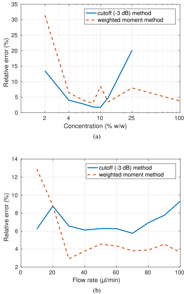
Fig. 7. Relative error of the cutoff frequency method (blue solid line) and the weighted moment approximation (red dashed lined) with regard to the value expected from equation (1). (a) Against milk concentration ratios by averaging the values obtained at each flow rate and (b) against flow rate by averaging the value obtained for each milk concentration except for concentration ratio lower than 4% for the weighted moment method and above 25% for the cutoff frequency method.
