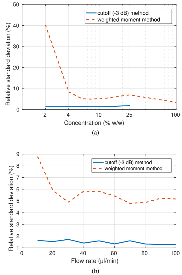
Fig. 8. Relative standard deviation for the cutoff frequency method (blue solid line) and the weighted moment approximation (red dashed lined) with regard to the value expected from equation(1). (a) Against milk concentration ratios by averaging the values obtained at each flow rate and (b) against flow rate by averaging the value obtained for each milk concentration except for concentration ratio lower than 4% for the weighted moment method and above 25% for the cutoff frequency method.
