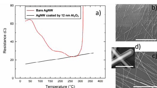
Figure 4. (a) In-situ measured resistance versus temperature of a AgNW network (deposited by spray-coating) during a thermal ramp showing that when a 12 nm thick layer of \text{Al}_2\text{O}_3 is deposited by SALD on AgNWs, a clear stability enhancement is observed since the network can undergo a thermal ramp up to 315 °C for bare AgNW and at least up to 370 °C for coated AgNW. For the coated network, the metallic behaviour can be observed through the linear increase of the electrical resistance with temperature associated to electron-phonon interactions. The SEM pictures are associated to bare AgNW (b) and coated AgNW (c) with 12 nm of \text{Al}_2\text{O}_3 . The SEM picture (d) corresponds to a higher resolution of a AgNW network coated with 43 nm of \text{Al}_2\text{O}_3 , where the coating can be clearly seen. Scale bars are 10 \mu\text{m} for (b) and (c) and 500 nm for (d). AgNWs have an average diameter of 90 nm and lengths between 10 to 20 \mu\text{m} , and the associated areal value of the network is about 85 \text{mg}/\text{m}^2 .
