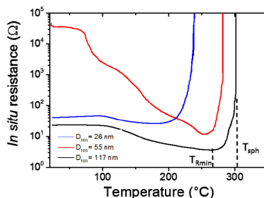
Figure 2. Evolution of the electrical resistance ( R ) of networks deposited by spin-coating and composed of AgNW with different average diameters ( D_{NW} ) during a 2^\circ\text{C}\cdot\text{min}^{-1} thermal ramp in air. One can clearly observe that the smaller the diameter, the lower the characteristic temperature, in agreement with Equation (2).
