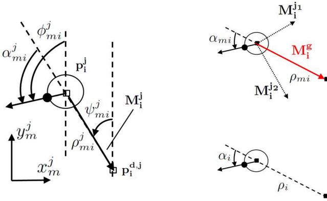
Fig. 3. Left: geometric variables and control vector computed for robot i by unit j , defined in its image. Right-top: representation of i 's global motion vector computed from image information received from two units j_1 and j_2 . Right-bottom: state of the robot on the ground plane.
