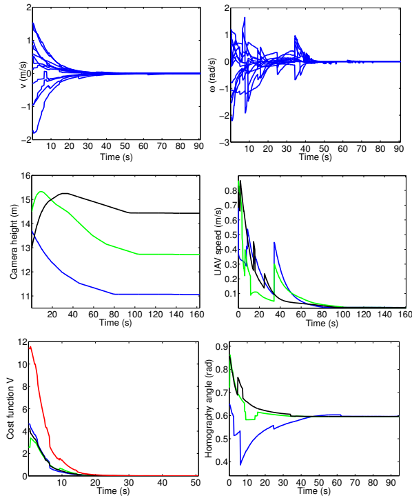
Fig. 7. Results from the realistic simulation. Top: Linear (left) and angular (right) velocities followed by the robots. Middle row: Evolution of the camera heights (left) and magnitudes of the UAV velocities (right). Bottom: cost functions for the cameras (the curve having greater values is the global Lyapunov function) (left), and angles of the cameras' 2D rotational homographies, expressed in a common frame (right).
