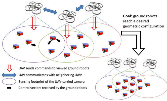
Fig. 1. Overview of the proposed multirobot control system.
