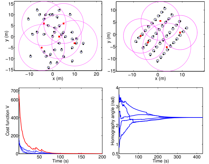
Fig. 5. Simulation results with forty robots and five cameras. Top: Initial (left) and final (right) configurations, showing the robots (circles), the cameras (squares), and the circular footprints associated with their field-of-view. Bottom: cost functions for every camera, and Lyapunov function, shown in a thicker line (left). Angles of the 2D rotational homographies computed by every camera, in a common reference frame (right).
