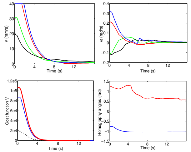
Fig. 8. Results from the experiment with real robots. Top row: Linear (left) and angular (right) velocities sent to the four robots. Bottom row: cost functions for the two cameras (the dashed line corresponds to the moving camera), and global Lyapunov function V (thicker line) (left). Evolution of the angle of the 2D rotational homography computed by the two cameras. The positive-valued curve corresponds to the moving camera (right).
