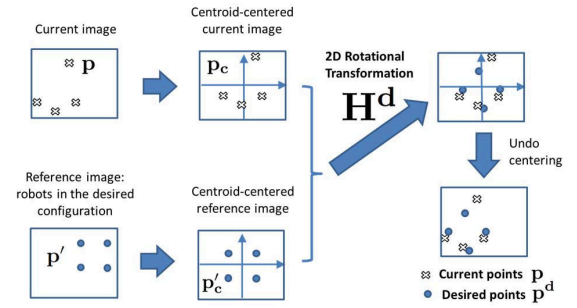
Fig. 2. Overview of the vision-based framework implemented by each of the control units using its associated camera. The computed desired image positions \mathbf{p}^d for the robots are such that the sum of their squared distances to the current positions \mathbf{p} is minimum, as explained in the text. The image-based control scheme we propose is based on driving \mathbf{p} to \mathbf{p}^d .
