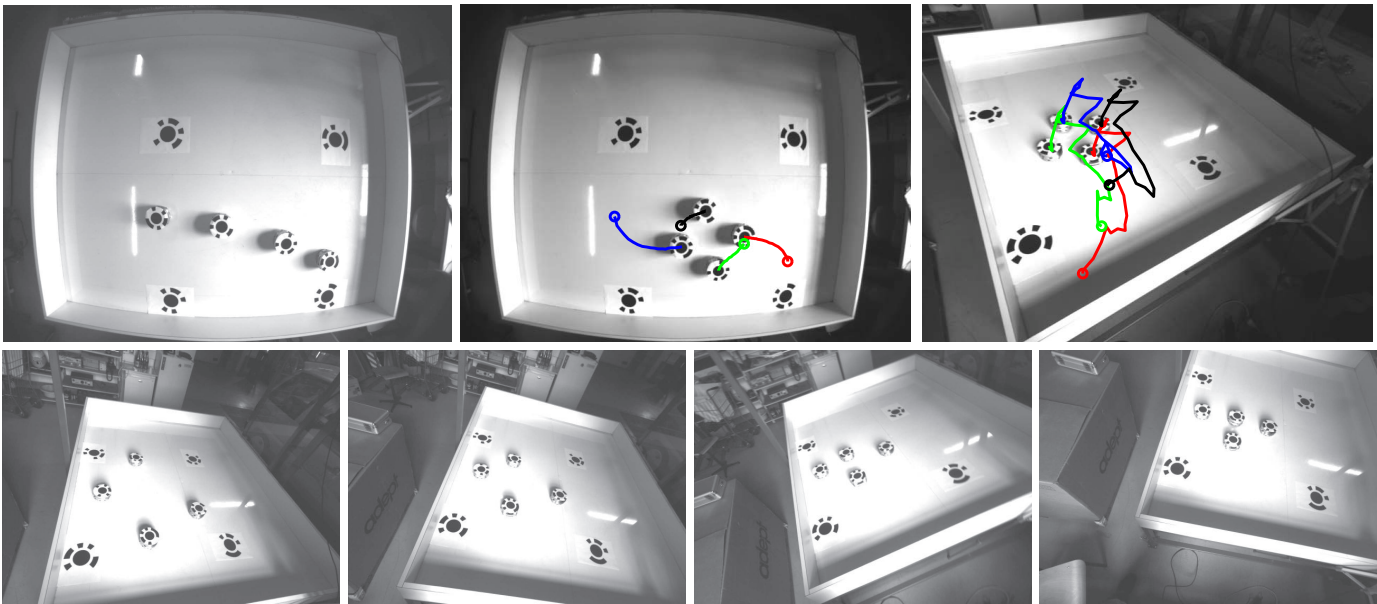
Fig. 9. Results from real experiments. The desired formation has the shape of a square (top row) and a "T" (bottom row). Top row: Initial image from the fixed camera (left). Final image from the fixed camera, with the image traces of the robots during the control execution overlaid (center). Final image, with the robots' image traces overlaid, for the moving camera (right). Bottom row: sequence of images from another experiment. The initial image (left), the final one (right) and two intermediate images from the moving camera are displayed.
