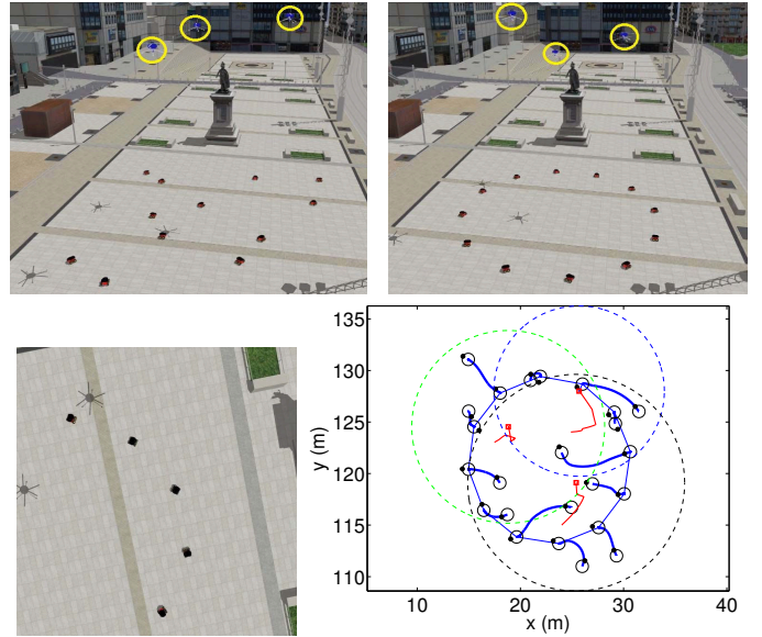
Fig. 6. Results from the realistic simulation example. Top: Initial (left) and final (right) views of the simulated setting, with circles plotted around the UAVs. Bottom: Final image captured by one of the cameras (left). Paths followed by the robots (right). The cameras' paths are displayed in thin lines, and their final positions are marked with squares. The final camera footprints are shown as dashed-line circles.
