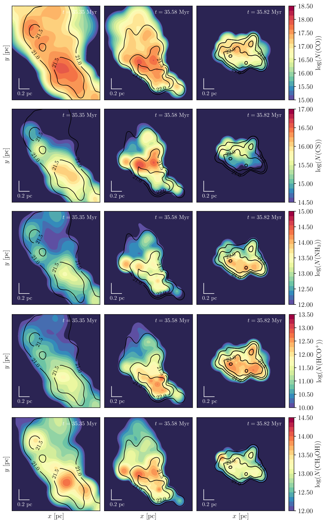
Fig. 3. Computed gas-phase column density maps of CO, CS, \text{NH}_3 , \text{HCO}^+ , \text{CH}_3\text{OH} at t = 35.35 Myr, t = 35.58 Myr, and t = 35.82 Myr for cloud A. Contours were added for clarity and indicate \log(N_{\text{H}}) from 21 to 23.
