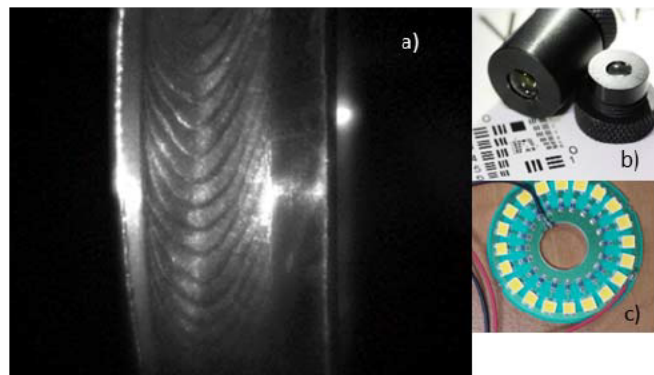
Fig. 1. (a) 600 nm monochromatic picture of a representative ITER welded steel ring. (b) FURHIS developed OS color (left) and monochrome (right). (c) Developed FURHIS IS architecture.
