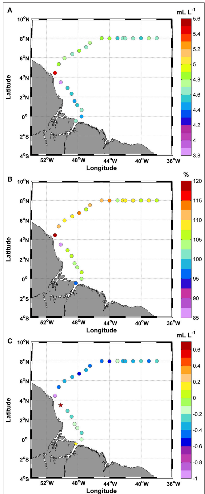
FIGURE 4 | Distributions of (A) Dissolved oxygen (DO); (B) Saturation of DO (%); and (C) Apparent oxygen utilization (AOU) along the ship track during the CF3 cruise, October 2012.
