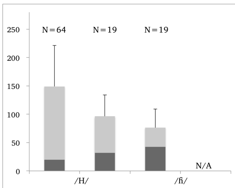
Figure 13. Mean duration and voicing period in /H/ and /ɦ/ in Xumi (in ms). Each bar is split into voiceless phases (grey) and voiced phases (black). /H/ is represented by two bars: the bar on the left stands for words spoken in isolation, the bar on the right stands for the same words occurring in sentences. The data for /ɦ/ are only from words in isolation. Error bars represent standard deviation of the mean value. The number of tokens is given above each bar.
