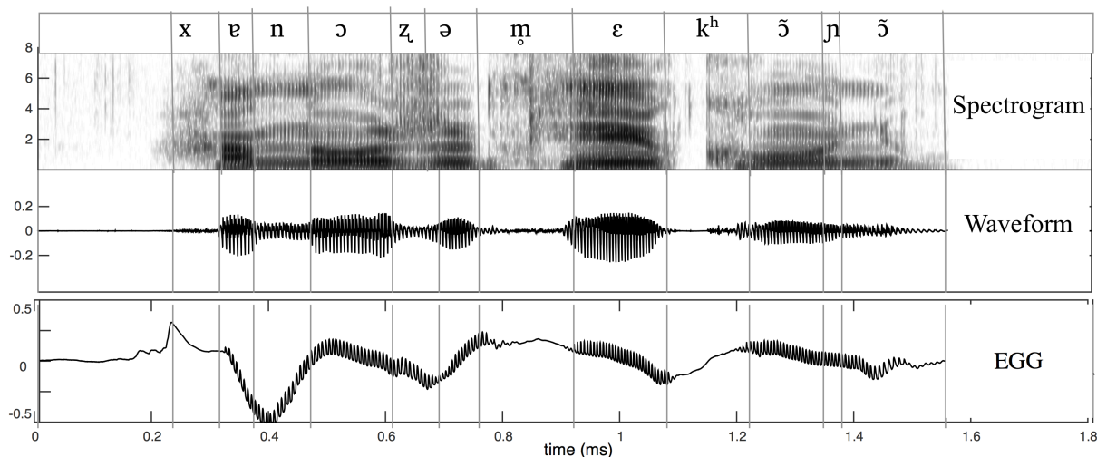
Figure 4: Spectrogram, waveform, and electroglottographic (EGG) signal for the Xumi sentence /xɛ 33 nɔ 33 =zə 55 m̥ɛ 55 kʰɔ̃ 55 ɲɔ̃ 31 / this.LOC=TOP medicine.house COP ‘This is a hospital.’
