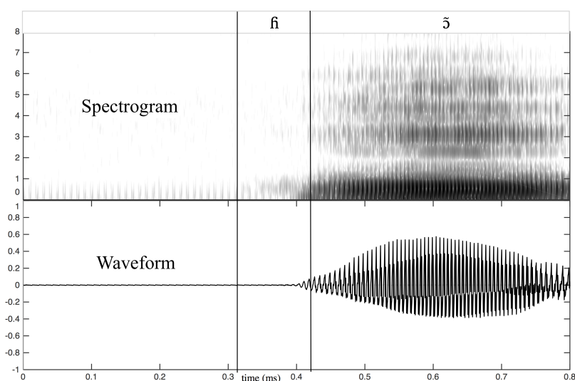
Figure 3a. A zoomed-in view of the consonant-vowel boundary in the Xumi word /fĩ 55 / ‘dare’
