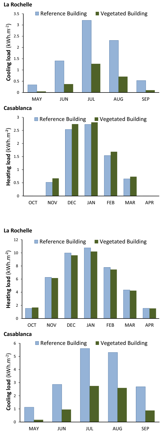
Fig. 8. Comparison between cooling and the heating thermal loads for the reference building and for the vegetated building in La Rochelle (France) and in Casablanca (Morocco).
