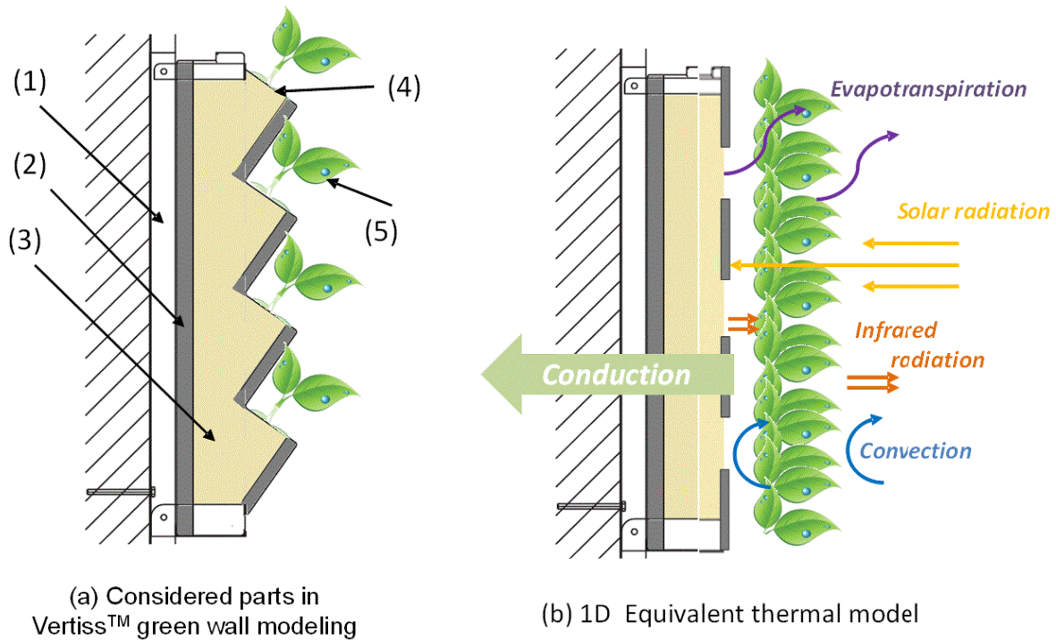
Fig. 5. Considered parts in Vertiss™ green wall modeling. (a) Considered parts in Vertiss™ green wall modeling. (b) 1D Equivalent thermal model.
