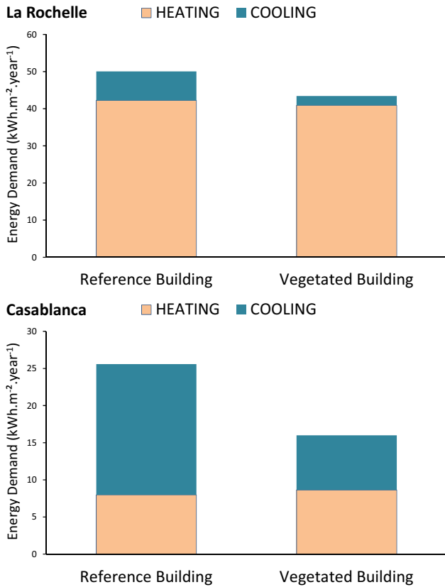
Fig. 7. Comparison between annual thermal loads for the reference building and for the vegetated building in La Rochelle (France) and Casablanca (Morocco).
