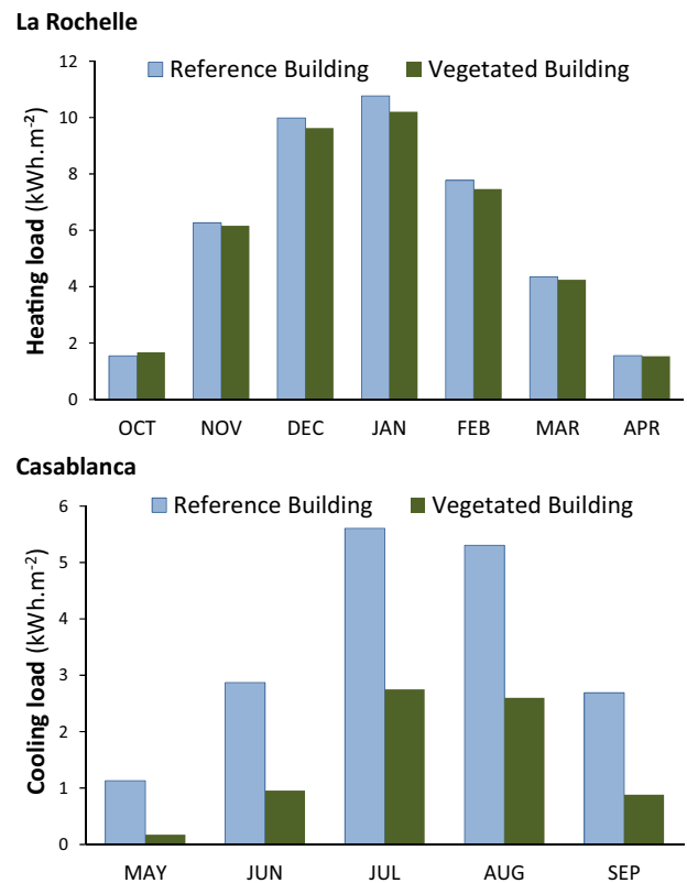
Fig. 8. Comparison between cooling and the heating thermal loads for the reference building and for the vegetated building in La Rochelle (France) and in Casablanca (Morocco).
