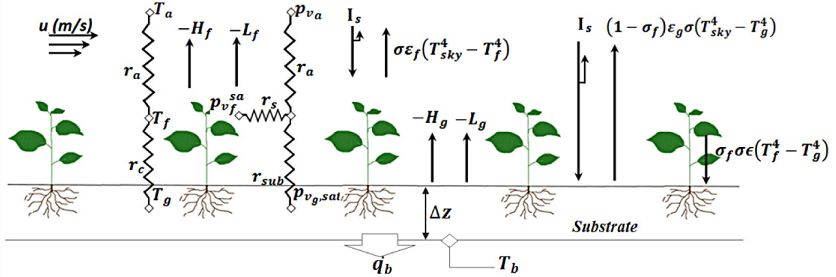
Fig. 1. Main modeled heat fluxes on a vegetated envelope module and corresponding heat and vapor transfer resistances.
