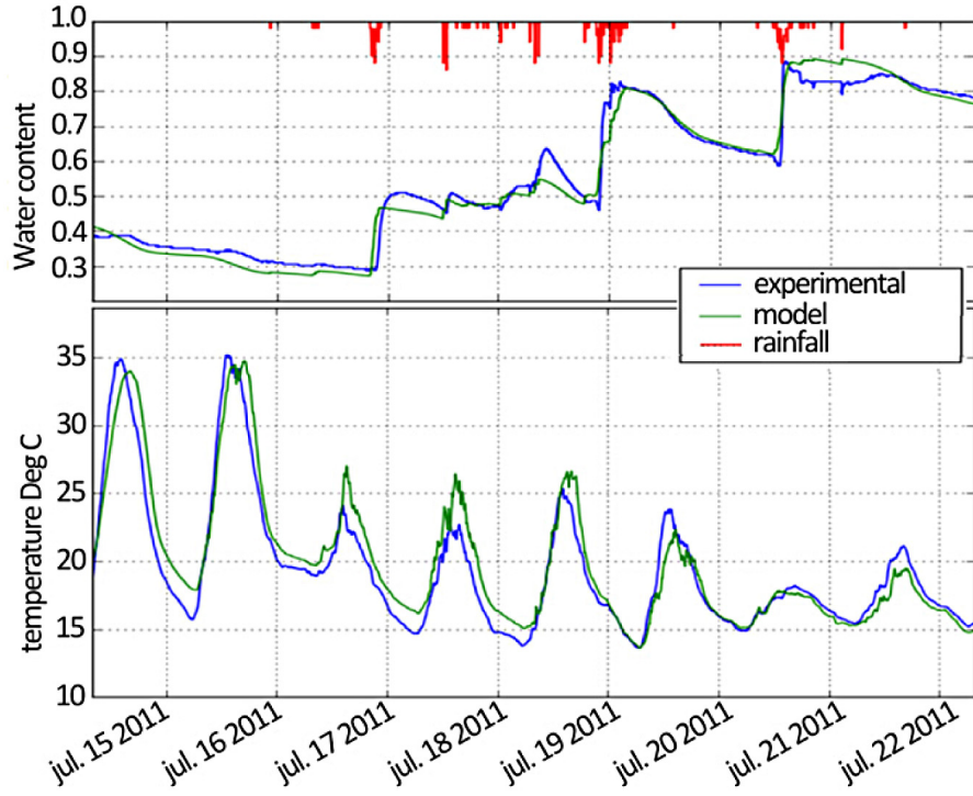
Fig. 2. Comparison between the numerical and the experimental temperature and water content results for a monitored green roof.
