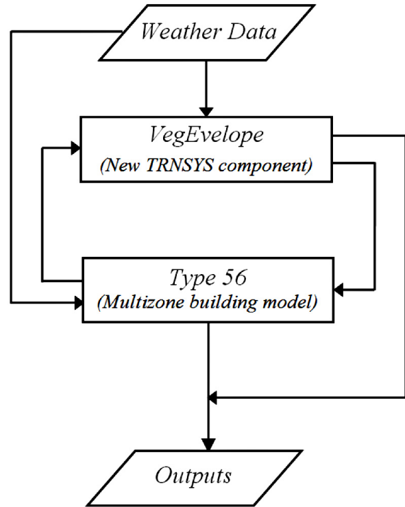
Fig. 3. Coupling the multizone building model with the new green envelope component in TRNSYS.
