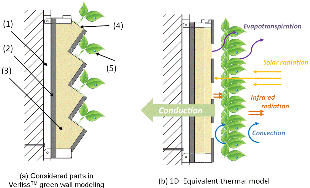
Fig. 5. Considered parts in Vertiss TM green wall modeling. (a) Considered parts in Vertiss TM green wall modeling. (b) 1D Equivalent thermal model.
