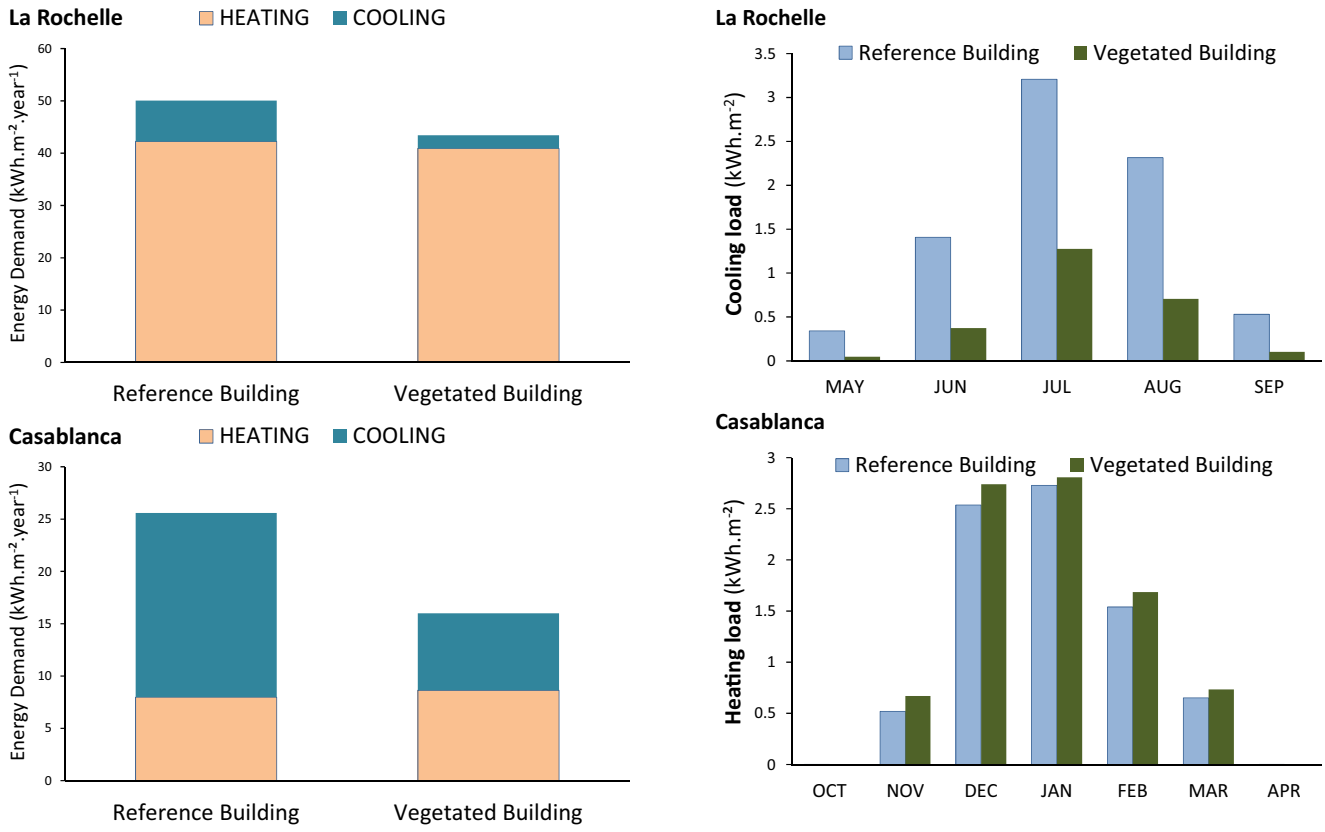
Fig. 7. Comparison between annual thermal loads for the reference building and for the vegetated building in La Rochelle (France) and Casablanca (Morocco).
