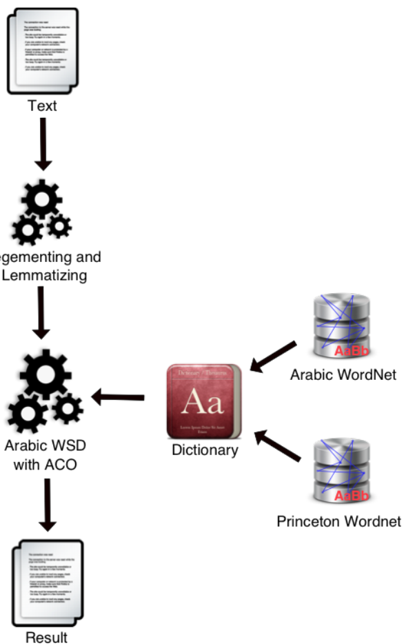
Fig. 2 Diagram of the proposed approach for AWSD
