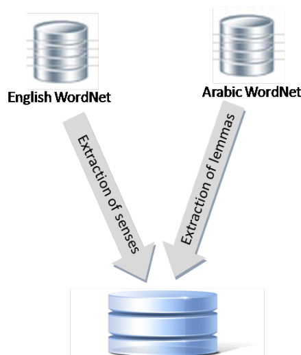
Fig. 1 Arabic Dictionary
