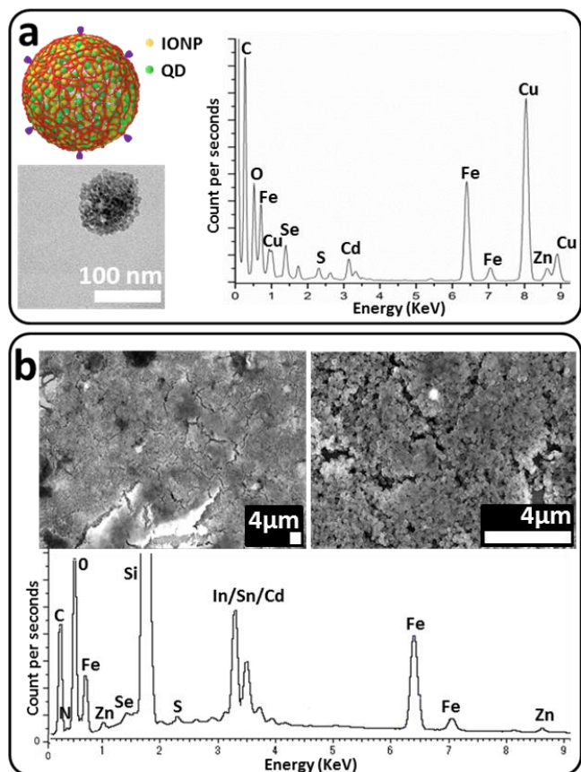
Figure 3: Chemical composition of films based on QD-containing Hybridosomes®. a) Schematic depiction, TEM micrograph and corresponding EDX analysis of Hybridosome nanocapsules composed of CdSe@ZnS quantum dots (green), IONPs (yellow) and PAA-C≡CH (red). b) SEM micrographs and EDX analysis of the corresponding films obtained after 800 CV cycles (-0.2 V to 0.6 V vs Ag/AgCl, 50 mV/s) in the presence of 4.5 \times 10^9 Hybridosomes/mL, 0.1 mg/mL N_3 -PEG- N_3 and 0.6 mM CuSO_4 at pH 3.5.
