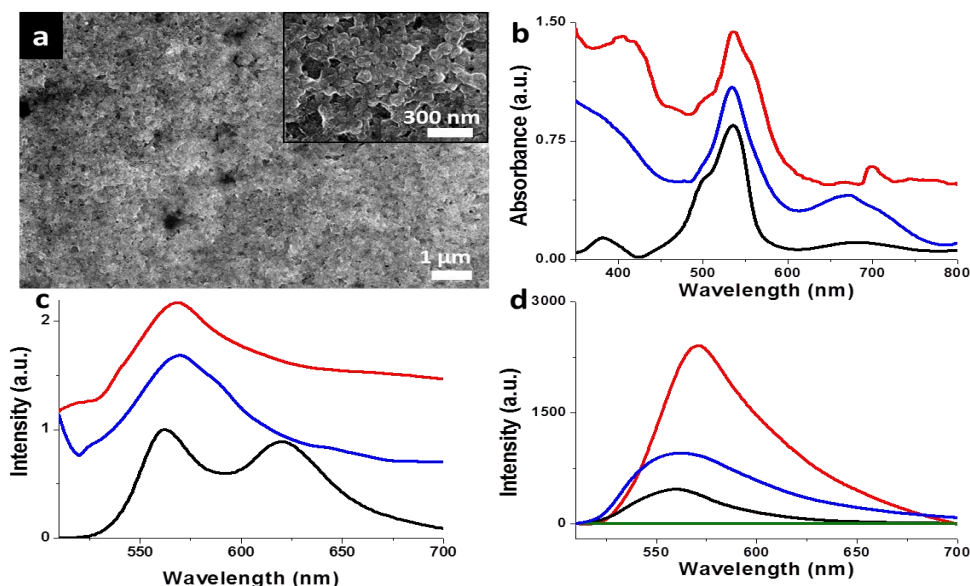
Figure 4: Bodipy-encapsulating Hybridosome® films. a) Typical SEM micrographs of bodipy-loaded Hybridosome films after 800 CV cycles. (b) UV-Visible absorbance spectra and (c) fluorescence spectra in the dry state ( \lambda_{exc} at 480 nm) of bodipy (black line), drop-casted bodipy-loaded Hybridosome (blue line) and an electro-clicked film based on bodipy-loaded Hybridosomes (red line). (d) Fluorescence spectra in the dry state ( \lambda_{exc} at 480 nm) of electro-clicked Hybridosome films obtained from building mixtures containing 0% (green line), 10% (black line), 50% (blue line) and 90% (red line) of bodipy-loaded Hybridosomes.
