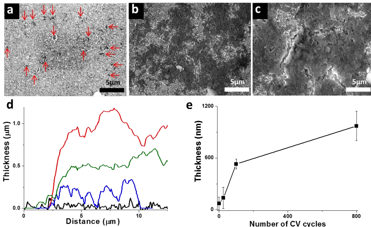
Figure 2: Germination and growth of covalently reticulated Hybridosomes® films. SEM micrographs of Hybridosome films on FTO after 25 (a), 100 (b) and 800 (c) CV cycles (-0.2 V to 0.6 V vs Ag/AgCl, 50 mV/s) in the presence of 4.5 \times 10^9 Hybridosomes/mL, 0.1 mg/mL N_3 -PEG- N_3 and 0.6 mM CuSO_4 at pH 3.5. d) Cross-sectional profiles of Hybridosome films, measured by AFM in the dry state and contact mode, after 0 (black line), 25 (blue line), 100 (green line) and 800 (red line) CV cycles. e) Evolution of the thickness of the corresponding films in the dry state
