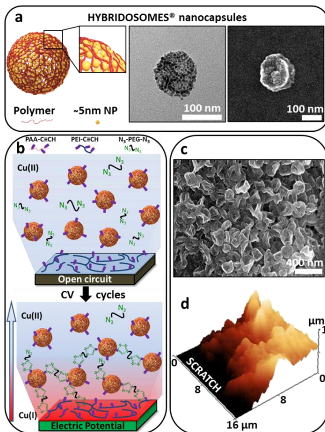
Figure 1: Concept of Hybridosomes ® films covalently assembled by using electro-click chemistry. a) Schematic depiction, TEM and SEM of deflated Hybridosome nanocapsules composed of iron oxide nanoparticles (IONPs) and polyacrylic acid. b) Schematic representation of the electro-click process, allowing the construction of films on PEI-C≡CH pre-coated electrodes, by using alkyne-functionalized Hybridosomes and azide homobifunctional PEG linkers as building blocks in the presence of electrogenerated Cu(I) catalyst. c) SEM micrograph of a typical Hybridosome film in the dried state. The film was constructed by electro-click after 800 CV cycles (-0.2 V to 0.6V vs Ag/AgCl, 50 mV/s) in the presence of 4.5 \times 10^9 Hybridosomes/mL, 0.1 mg/mL N 3 -PEG-N 3 and 0.6 mM CuSO 4 at pH 3.5. d) Typical 3D view of the corresponding scratched film measured by AFM in the dry state and contact mode.
