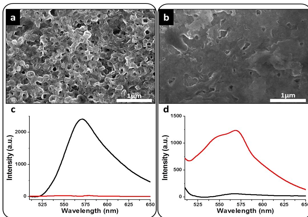
Figure 5: Electro-triggered release abilities of electro-clicked Hybridosomes® films. SEM micrographs (a, b) and fluorescence spectra ( \lambda_{\text{exc}} at 480 nm) in the dry state (c, d) of bodipy-loaded Hybridosome films assembled on FTO (black line) and of the corresponding supernatant (red line) before (a, c) and after (b, d) application of +1 V potential (vs Ag/AgCl) for 15 minutes in a 0.1M NaCl solution.
