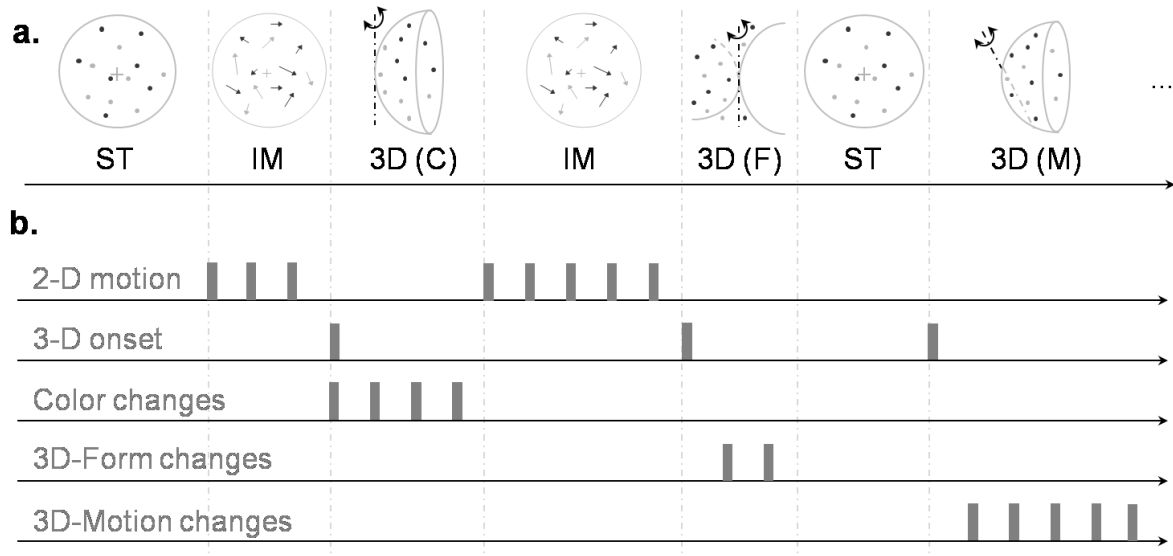
Figure 1: Experimental conditions and associated model of the BOLD response. (a) Stimulation sequence in passive viewing. The baseline consists of static dots (ST). Stimuli are either incoherent motion (IM) or three-dimensional surfaces (3D) changing colour (C), form (F) or motion direction (M) every 2s. (b) Onsets for the 5 event-related regressors modelling the fMRI signal. For the 2-D motion regressor, intervening onsets correspond to changes in local motion directions.
