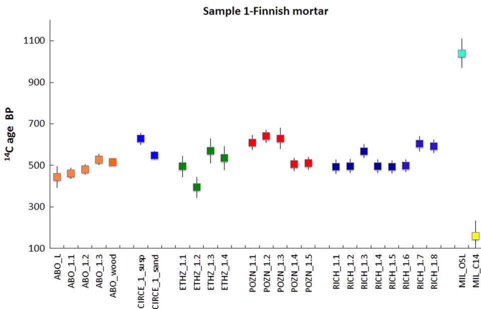
Figure 3 Sample of Finish mortar—the independent age was obtained on wood ABO_wood 512 ± 9 BP. Additional notes: L-lump, fractions of different dissolution steps (supplementary Table S1) are shown as LAB_1.2, LAB_1.3, etc. Results of each laboratory are shown in different colors (ordered as in Table 1; refer to online version for colors).
