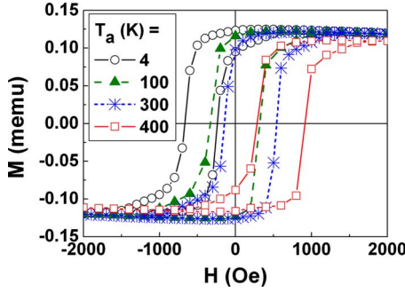
FIG. 2. (Color online) Hysteresis loops for films of Ta (3 nm)/Cu (3 nm)/Co (3 nm)/IrMn (7 nm)/Pt (2 nm), for different annealing temperatures ( T_a ). The samples were initially FC under a positive saturating field of 10 kOe from above T_{B,\max} down to 4 K. They were then FC under -10 kOe from T_a down to 4 K. The loops were recorded at 4 K by SQUID along the FC direction.
