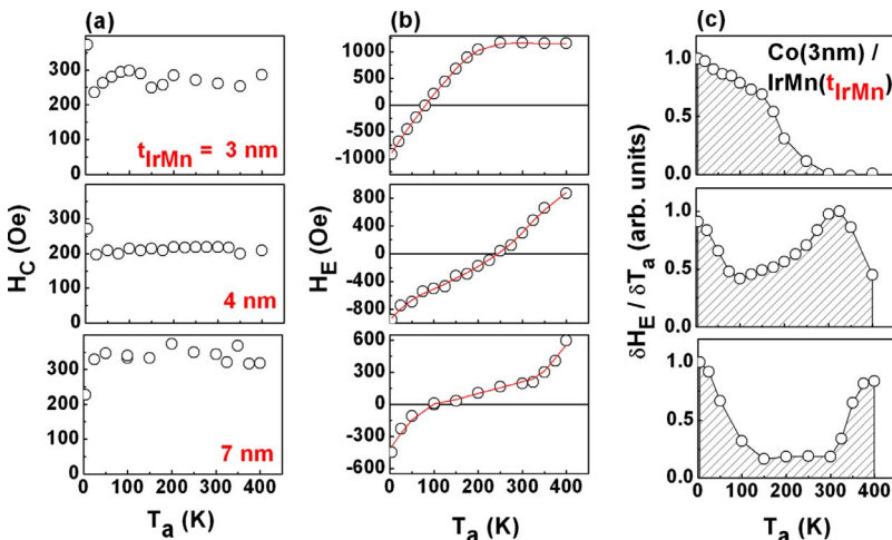
FIG. 3. (Color online) Dependence of (a) the coercive field ( H_C ), (b) EB field ( H_E ), and (c) derivative \delta H_E / \delta T_a on the annealing temperature ( T_a ) for Co (3 nm)/IrMn ( t_{IrMn} = 3, 4, and 7 nm) films. \delta H_E / \delta T_a vs T_a are the blocking temperature distributions. H_C and H_E are determined after hysteresis loops subsequent to cooling procedures described in the caption of Fig. 2. The lines in (b) result from smoothing of the raw data and were used for the derivative.
