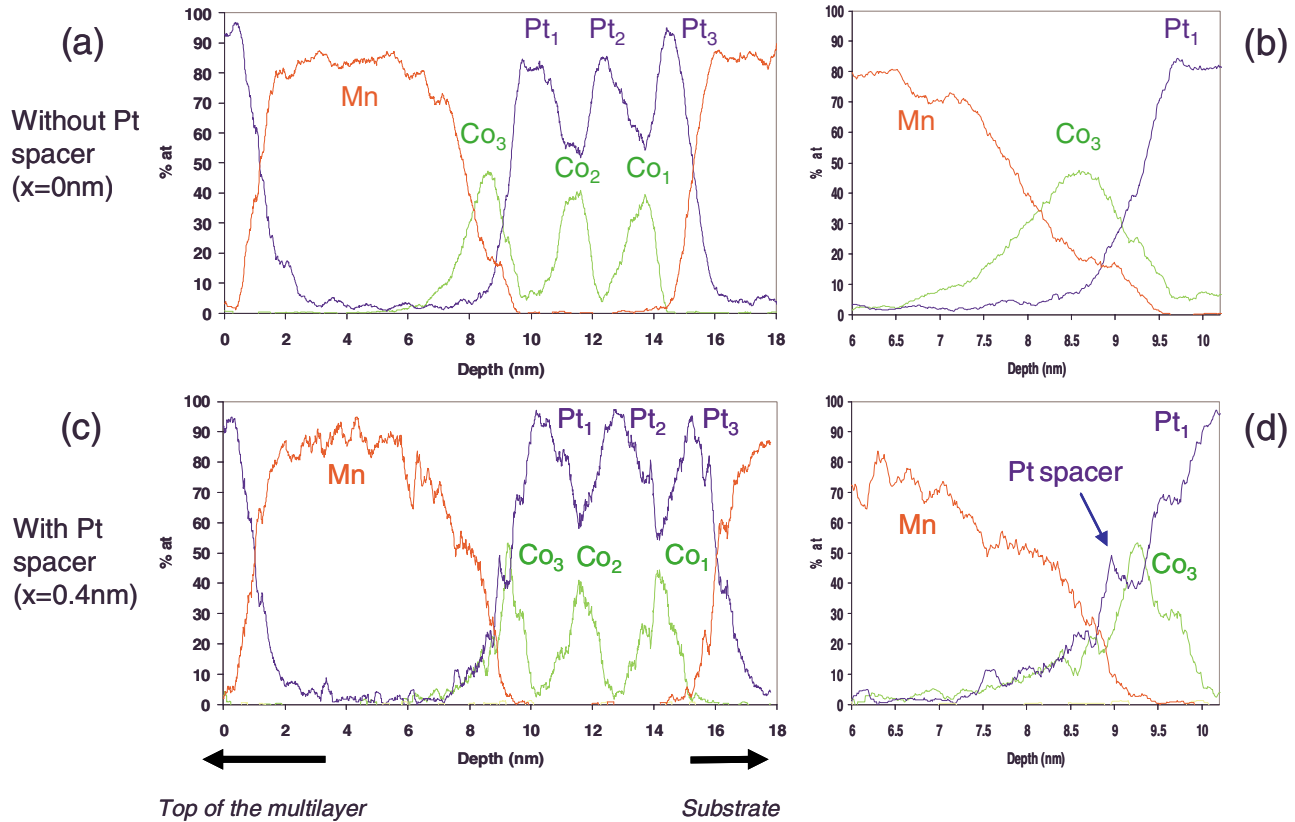
FIG. 2. (Color online) Concentration profiles of the Pt, Co, and Mn atoms corresponding to the 2D projection of one sequence of the [(\text{Pt}_2 \text{ nm}/\text{Co}_{0.4} \text{ nm})_3/\text{Pt}_x/\text{IrMn}_7 \text{ nm}] multilayers: [(a) and (b)] without Pt spacer ( x=0 \text{ nm} ) and [(c) and (d)] with Pt spacer ( x=0.4 \text{ nm} ). (b) and (d) are the enlargements of profiles close to the FM/AFM interface.
