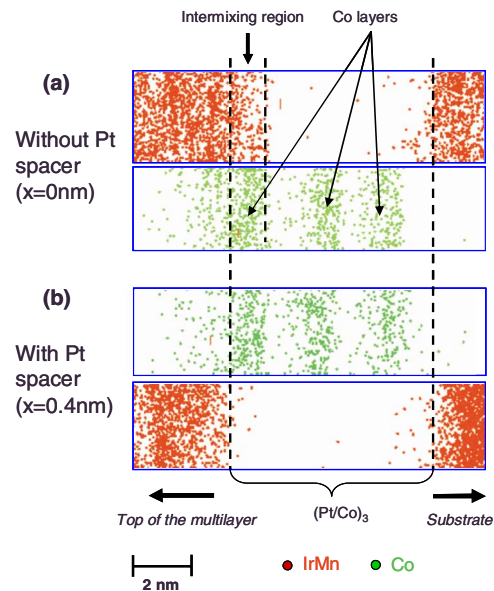
FIG. 1. (Color online) Two-dimensional (2D) projection of the analyzed volumes representing one sequence of the [(\text{Pt}_2 \text{ nm} / \text{Co}_{0.4 \text{ nm}})_3 / \text{Pt}_x / \text{IrMn}_7 \text{ nm}]_2 multilayers. (a) Without Pt spacer ( x=0 nm) and (b) with Pt spacer ( x=0.4 nm).
