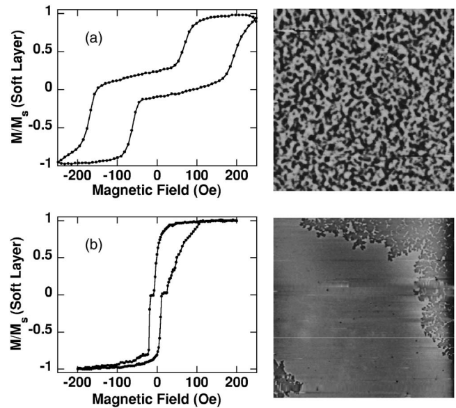
FIG. 4. Minor hysteresis loops and corresponding MFM images. (a) Sample demagnetized with a saturating in plane magnetic field ( 25 \times 25 \mu\text{m}^2 image). (b) Sample demagnetized at the coercive field of the hard layer ( 110 \times 110 \mu\text{m}^2 image).
