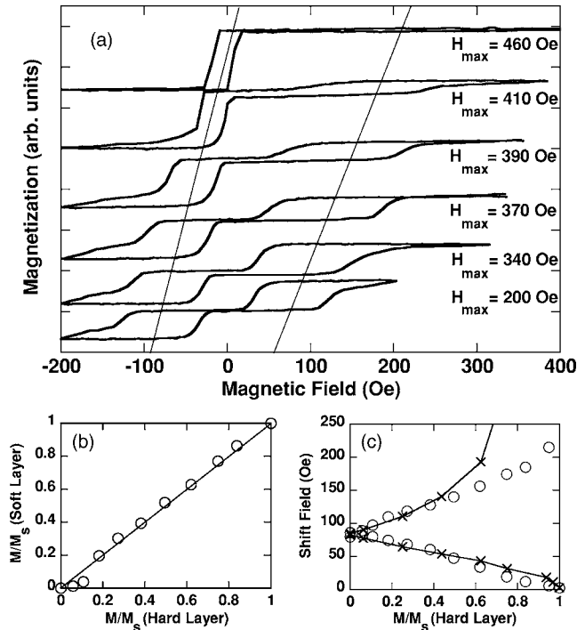
FIG. 3. (a) Hysteresis loops recorded with increasing the maximum positive applied field. Curves are shifted vertically for clarity. Oblique lines are a guide to the eyes and give the trend of variation of the loop shifts. (b) Variation of the net magnetization of the soft layer as a function of the net magnetization of the hard layer. (c) Variation of the shift fields as a function of the net magnetization of the hard layer. The solid line gives the variation of the calculated stray fields.
