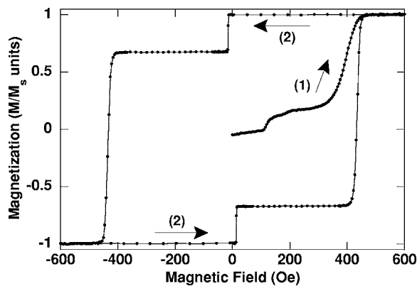
FIG. 1. First magnetization curve and major hysteresis loop obtained from Hall effect measurements. The magnetic field is applied perpendicular to the sample plane. The magnetization is normalized to the total magnetization of the sample. (1) is the first magnetization curve, and (2) is the major hysteresis loop.
