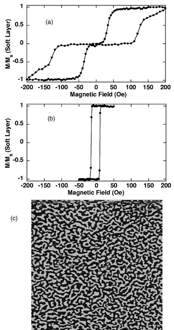
FIG. 2. Minor hysteresis loops for the soft layer. The hard layer is either (a) demagnetized or (b) saturated. The magnetization is normalized to that of the soft layer. (c) is a 110 \times 110 \mu\text{m}^2 MFM image in the demagnetized remanent state.
