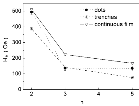
FIG. 4. Evolutions of the exchange bias field H_E with the number of Pt/Co repeats n for [\text{Pt}(2 \text{ nm})/\text{Co}(0.6 \text{ nm})]_n/\text{IrMn}(5 \text{ nm})/\text{Pt}(2 \text{ nm}) stacks.
