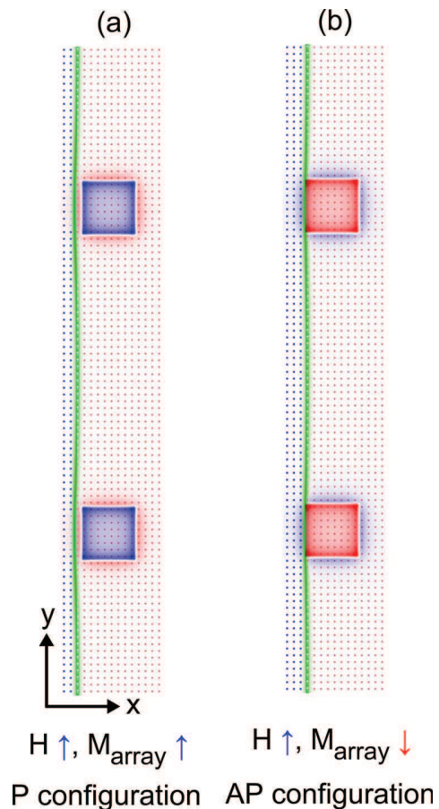
FIG. 3. Micromagnetic simulation ( 400 \text{ nm} \times 2400 \text{ nm} ) of domain walls propagating through an ideal (defect free) Co(0.65 nm) layer towards the location of two nanoplatelets for the (a) P configuration ( M_{array} \uparrow and H \uparrow ) and the (b) AP configuration ( M_{array} \downarrow and H \uparrow ). The perpendicular component of the field of the nanoplatelets within the calculation region has been superimposed on the image (the blue and red "squares"). The color code for the film's magnetization and the nanoplatelets' perpendicular dipolar fields is +z = \text{blue} , -z = \text{red} , and +y = \text{green} (Bloch domain wall).
