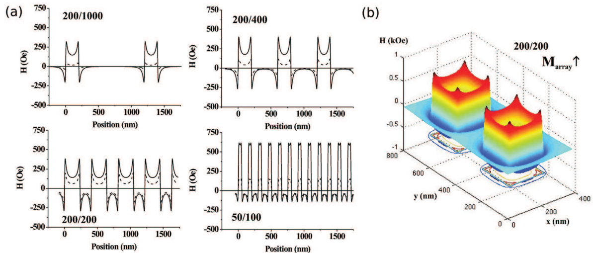
FIG. 2. (a) Perpendicular component of the stray field beneath positively saturated nanoplatelets ( \uparrow ) as calculated at the center of the soft layer in the 200/1000, 200/400, 200/200, and 50/100 arrays. The solid line represents the stray field value along a line passing through the center of a row of nanoplatelets. The dotted line corresponds to its value averaged over a moving window in the plane of the continuous layer with a width of 10 nm and a length equal to the array period. The latter allows one to visualize the field experienced by a straight wall moving through the array averaged along its length. (b) Plot of the perpendicular component of the nanoplatelet stray field for the 200/200 array beneath two neighboring nanoplatelets.
