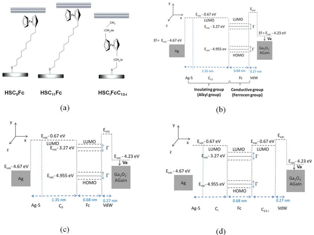
FIG. 1. (a) Schematic representation of molecular diodes made of ferrocenyl-containing alkanethiols. It consists of Ag bottom electrodes, SAM of \text{SC}_9\text{Fc} , \text{SC}_{11}\text{Fc} or \text{SC}_i\text{FcC}_{13-i} , and \text{Ga}_2\text{O}_3\text{-EGaIn} electrodes. The theoretical energy band diagram of molecular diodes made of (b) \text{HSC}_{11}\text{Fc} , (c) \text{HSC}_9\text{Fc} , and (d) \text{HSC}_i\text{FcC}_{13-i} .
