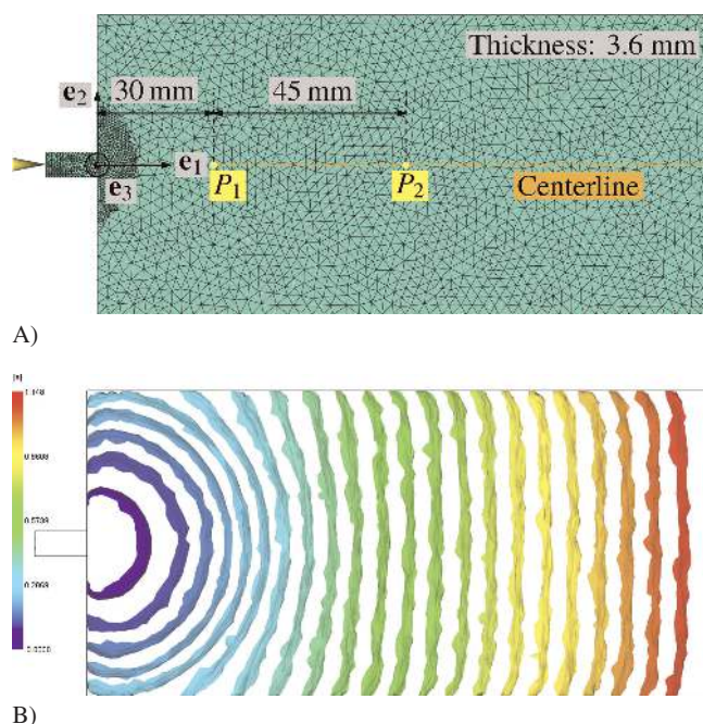
Fig. 6. Rectangular end-gated flat plate with two probe points (A), filling contour for the uncoupled and coupled injection simulations (B)
