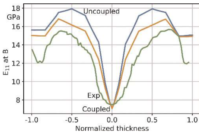
Fig. 21. Homogenized Young’s modulus E_{11} at B : comparison between the uncoupled/coupled simulations and experimental data
