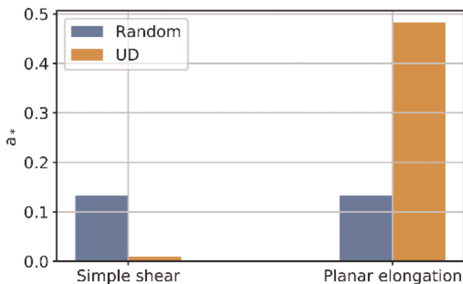
Fig. 3. Coupling factor a_* for two particular orientation states under two typical flows, for UD: \bar{a}_{11} = 0.98
