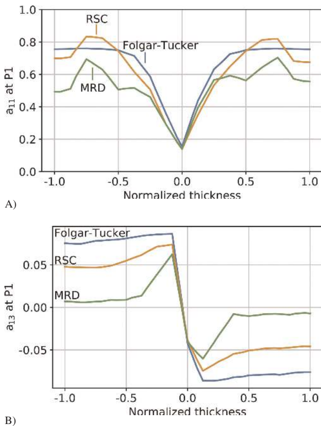
Fig. 7. Fiber orientation a_{11} (A) and a_{13} (B) at P1 for the Folgar-Tucker, RSC and MRD models without flow-viscosity coupling
