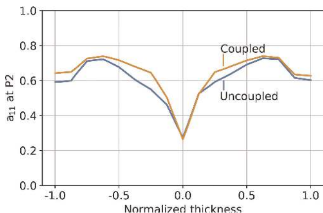
Fig. 9. Fiber orientation a_{11} at P1 (A) and P2 (B) probe points using the MRD model with or without flow-fiber coupling where \bar{a}_{11} = 0.93
