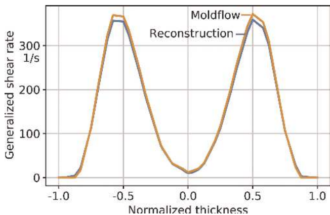
Fig. 14. Reconstruction of the generalized scalar shear rate at P1
