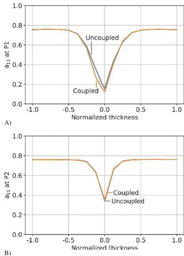
Fig. 8. Fiber orientation a_{11} at P1 (A) and P2 (B) probe points using the Folgar-Tucker model with or without flow-fiber coupling where \bar{a}_{11} = 0.93
