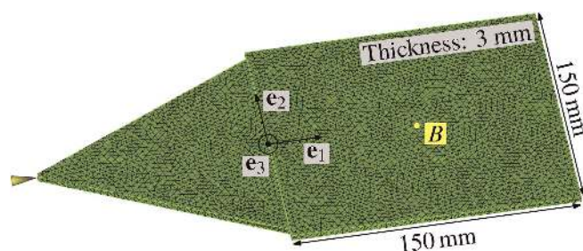
Fig. 19. Geometry of a fan-gated rectangular plate with one probe point located at the center
