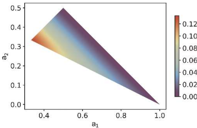
Fig. 2. Smallest eigenvalue of the 4th-order fiber orientation tensor approximated by the orthotropic closure formulation in the TUB orientation space
