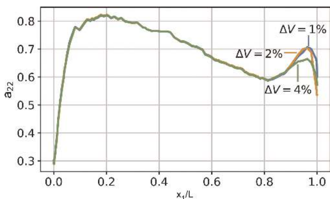
Fig. 5. Fiber orientation a_{22} on the midsurface along the length direction from the gate x_1/L = 0 up to the end x_1/L = 1 obtained for three different time-step increments, z = 0
