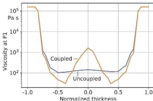
Fig. 10. Results obtained at the end of filling at P1 using the MRD model with or without flow-fiber coupling where \bar{a}_{11} = 0.93 : (A) velocity profile v_x ; (B) viscosity profile
