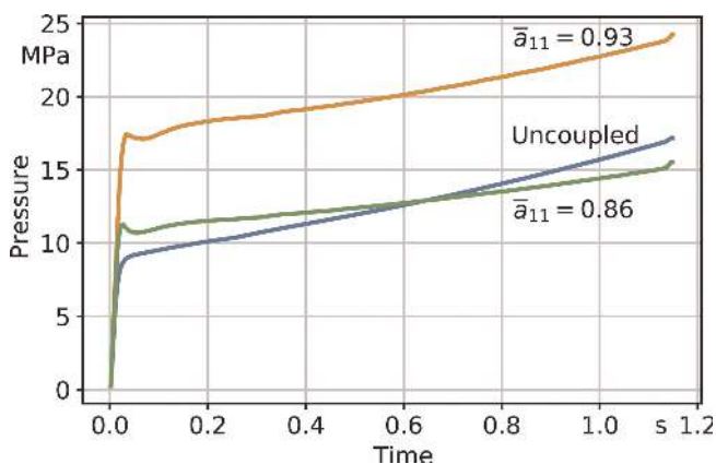
Fig. 18. Pressure at the injection point using the RSC model with flow-fiber coupling
