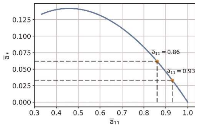
Fig. 4. Variation of \bar{a}_* as \bar{a}_{11} increases from 1/3 (isotropic state) to 1 (unidirectional state)
