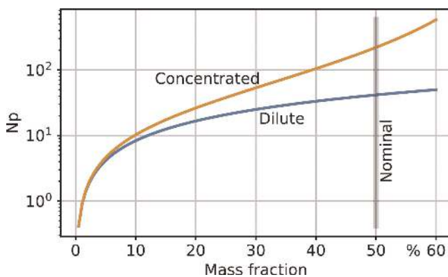
Fig. 1. Anisotropic contribution coefficient N_p for PA-GF50 as a function of the mass fraction using the dilute (Ericksen, 1959) and the concentrated (Phan-Thien and Graham, 1991) theories
