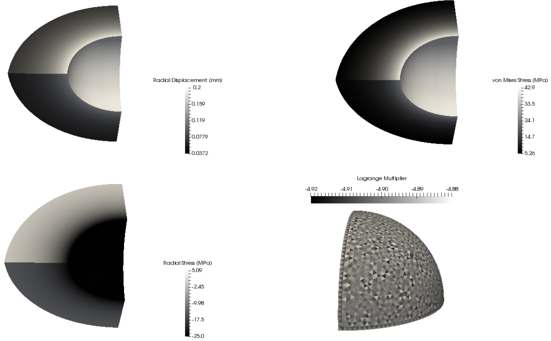
Figure 6: Numerical results obtained with LAC in 3D when considering 10-node tetrahedra. Top left : radial displacement; top right : Von Mises stresses; bottom left : radial stresses; bottom right : contact pressure
