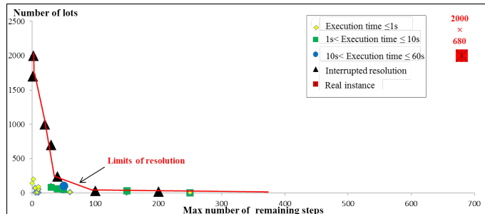
Fig. 3: Limits of MIP resolution.
