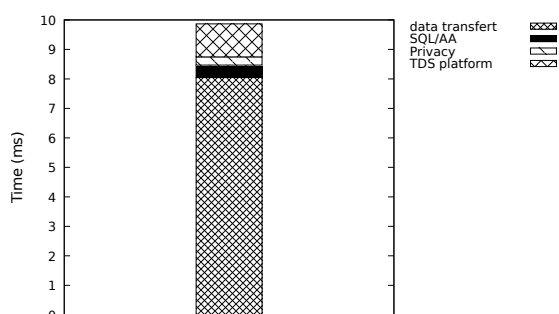
Figure 11: Filtering Phase Execution Time Breakdown.
