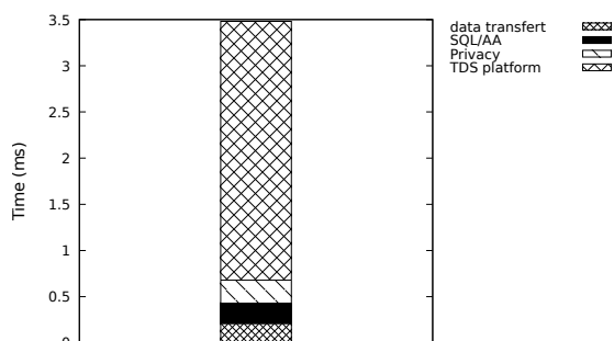
Figure 10: Collection Phase Execution Time Breakdown.
